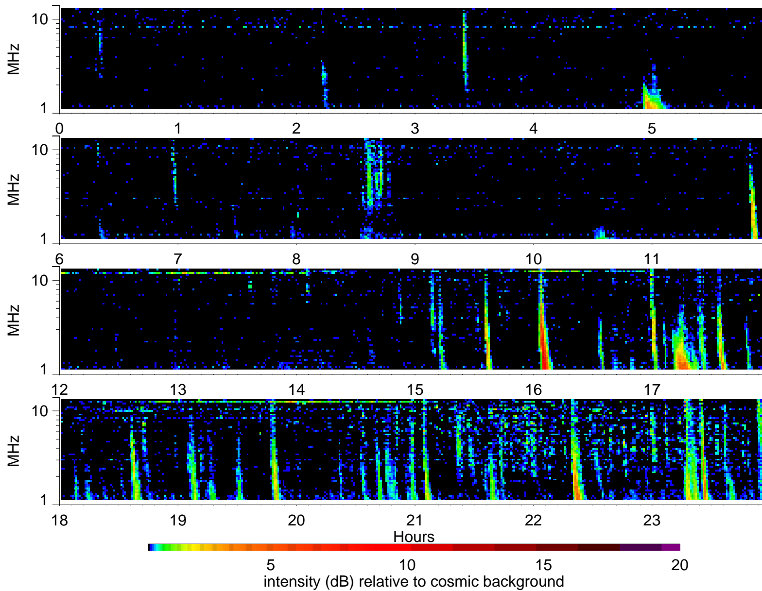
Wind Waves RAD2 receiver: 2003/4/3
