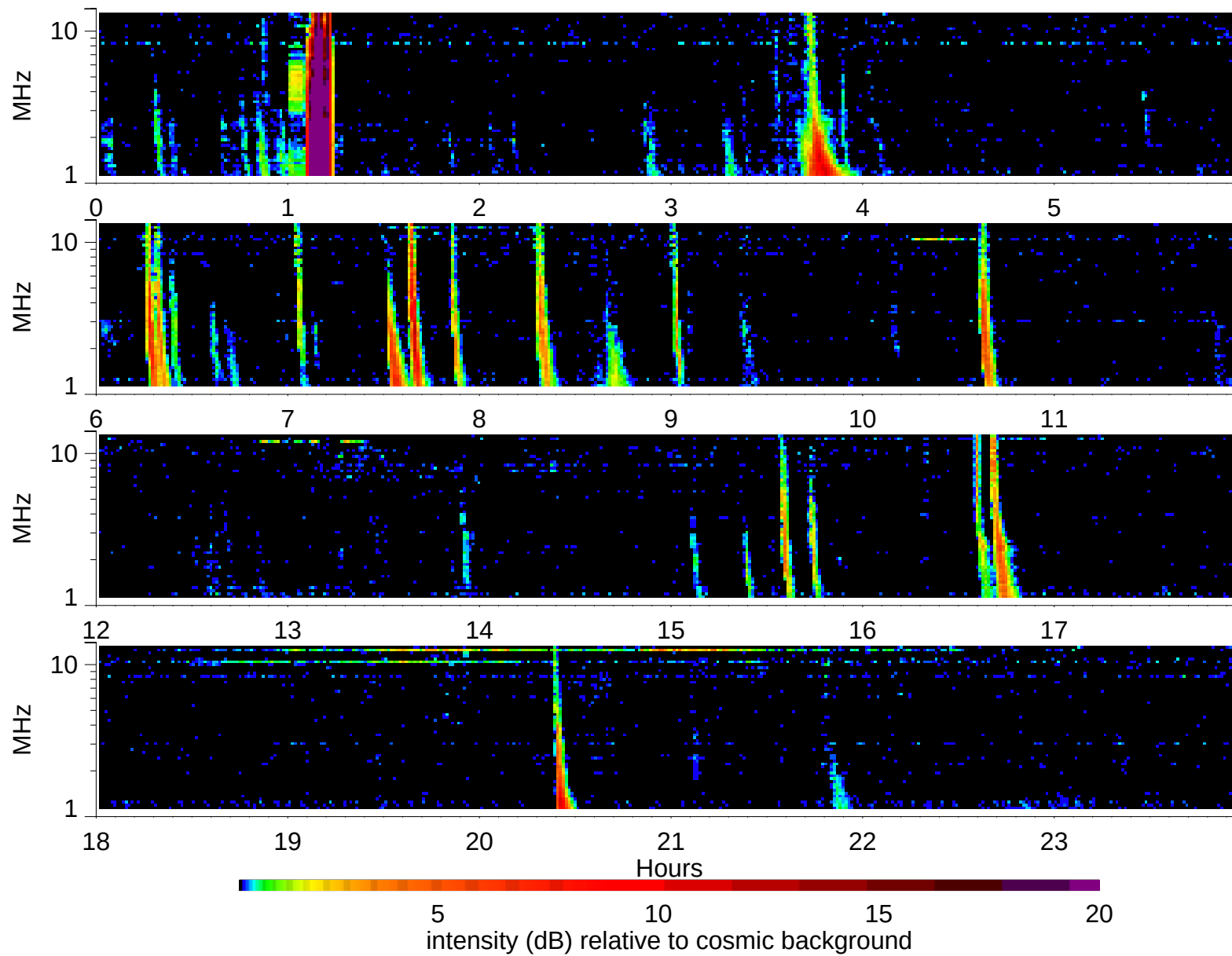
Wind Waves RAD2 receiver: 2003/4/2
