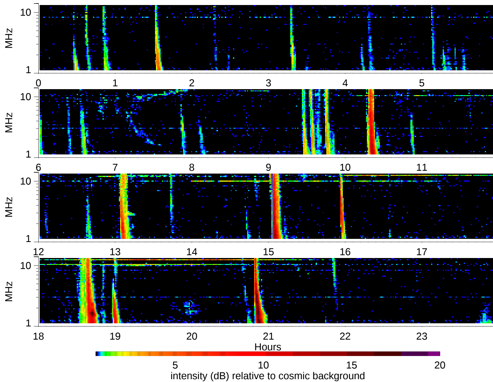
Wind Waves RAD2 receiver: 2003/3/29
