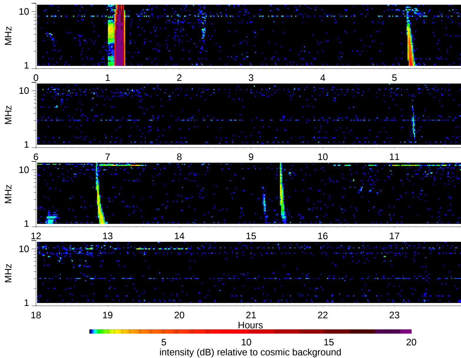
Wind Waves RAD2 receiver: 2003/3/25
