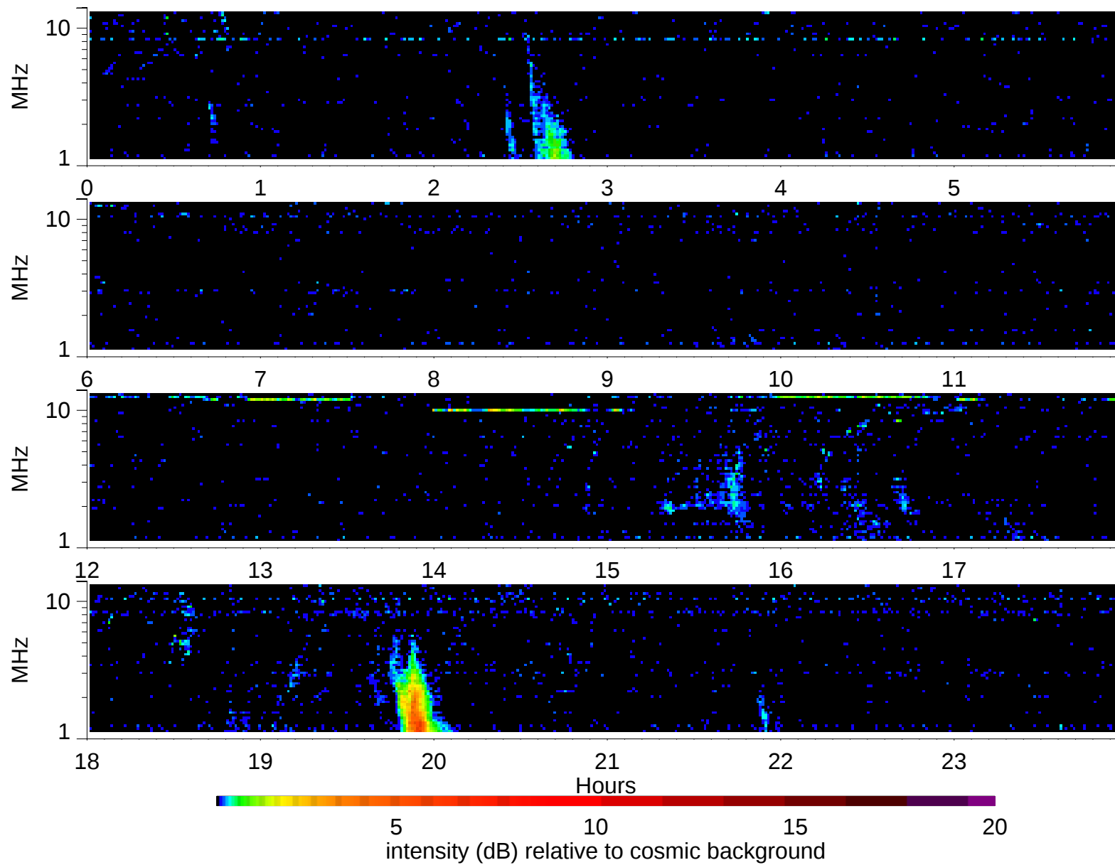
Wind Waves RAD2 receiver: 2003/3/24
