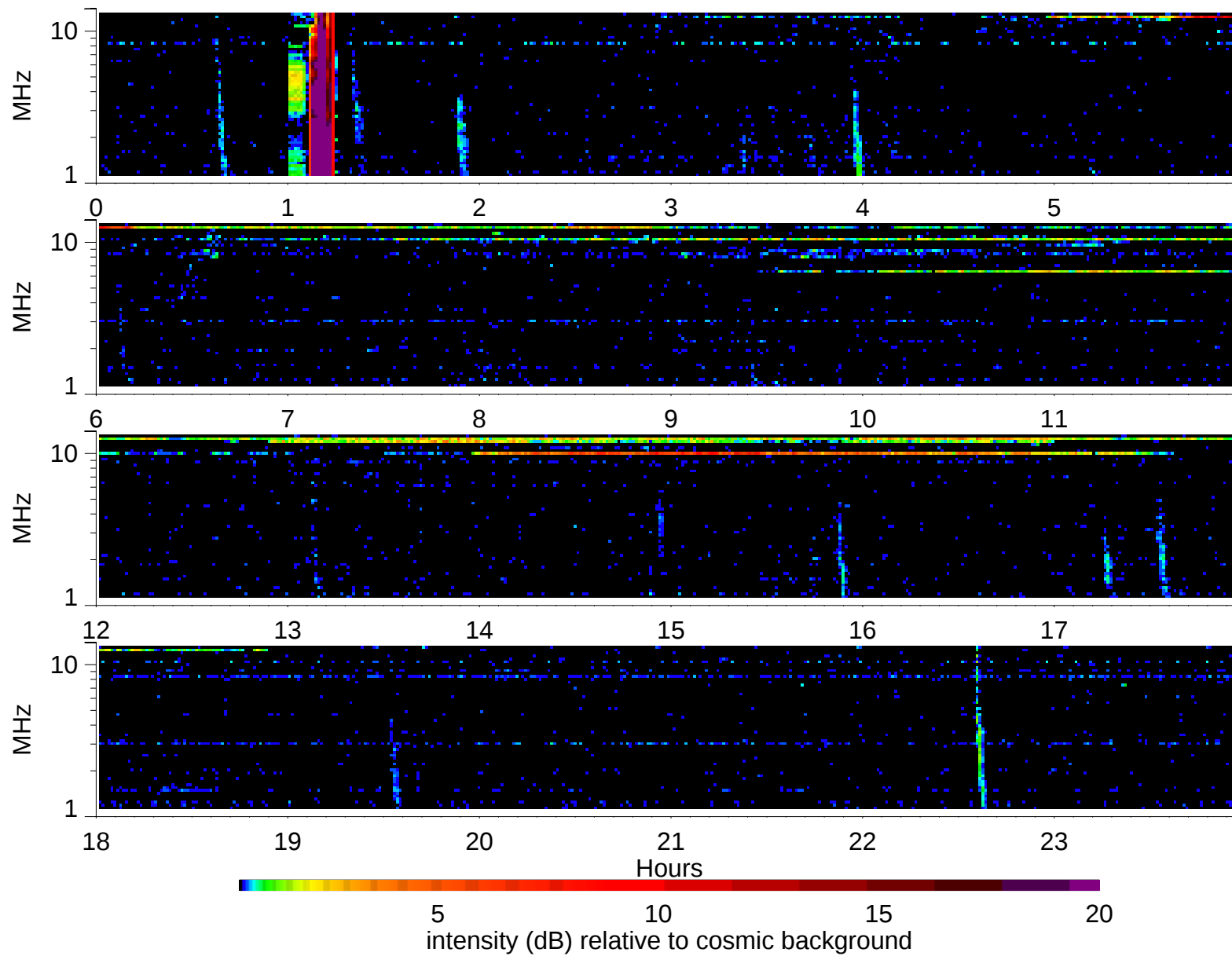
Wind Waves RAD2 receiver: 2003/3/21
