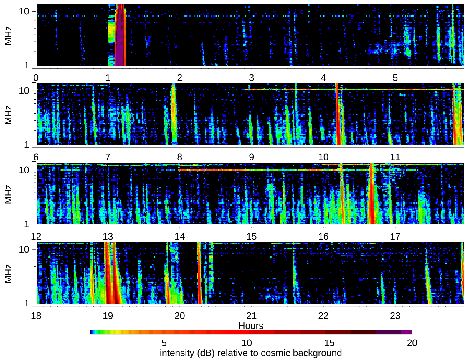
Wind Waves RAD2 receiver: 2003/3/17
