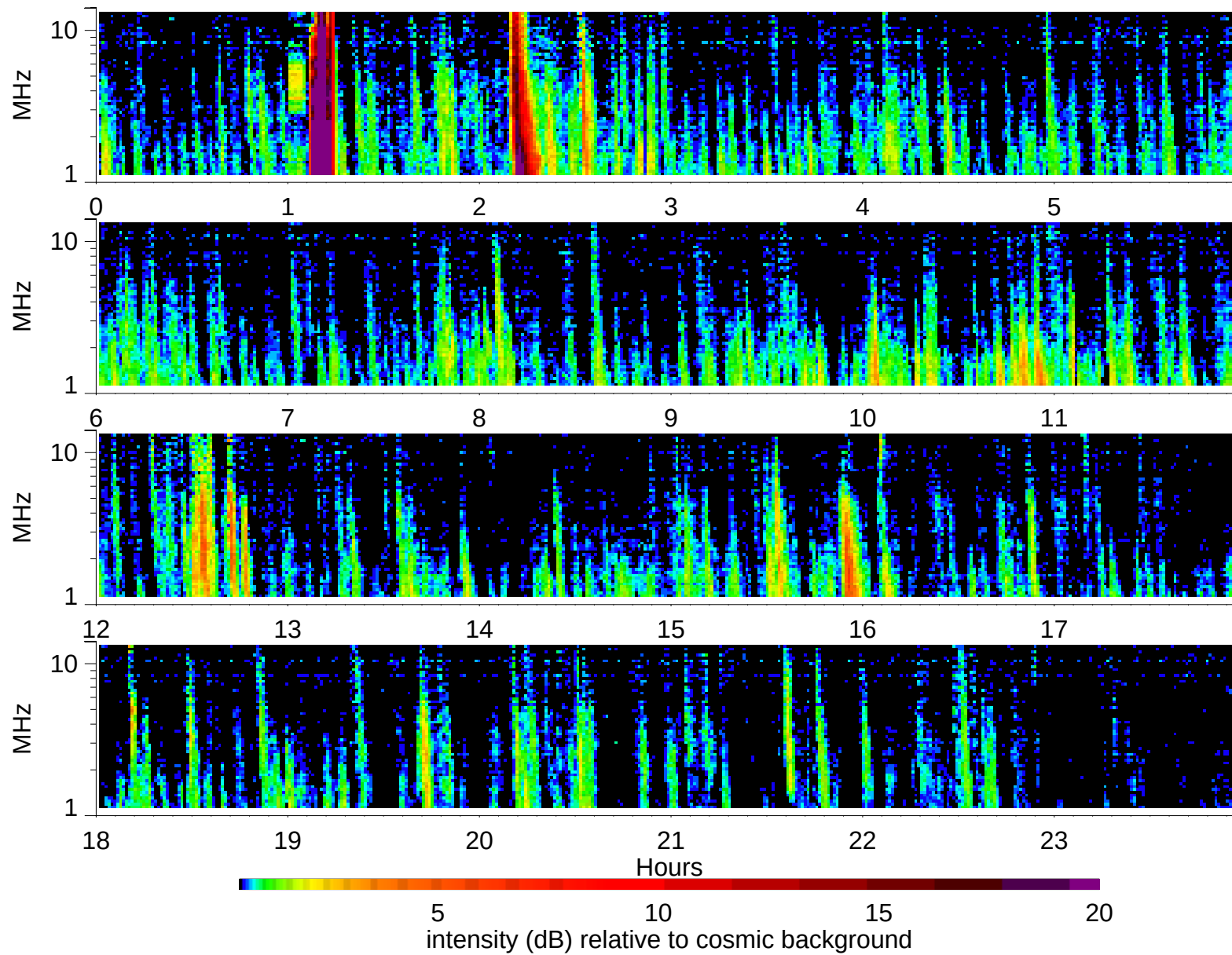
Wind Waves RAD2 receiver: 2003/3/13
