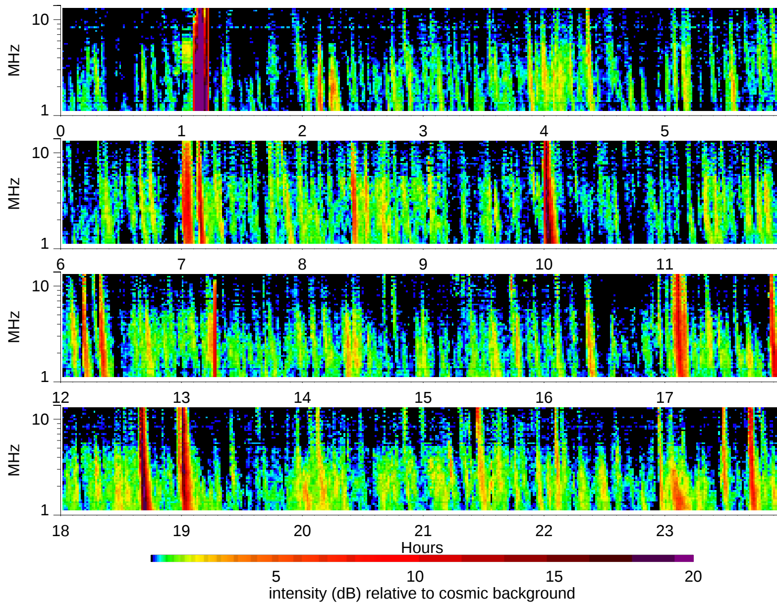
Wind Waves RAD2 receiver: 2003/3/11
