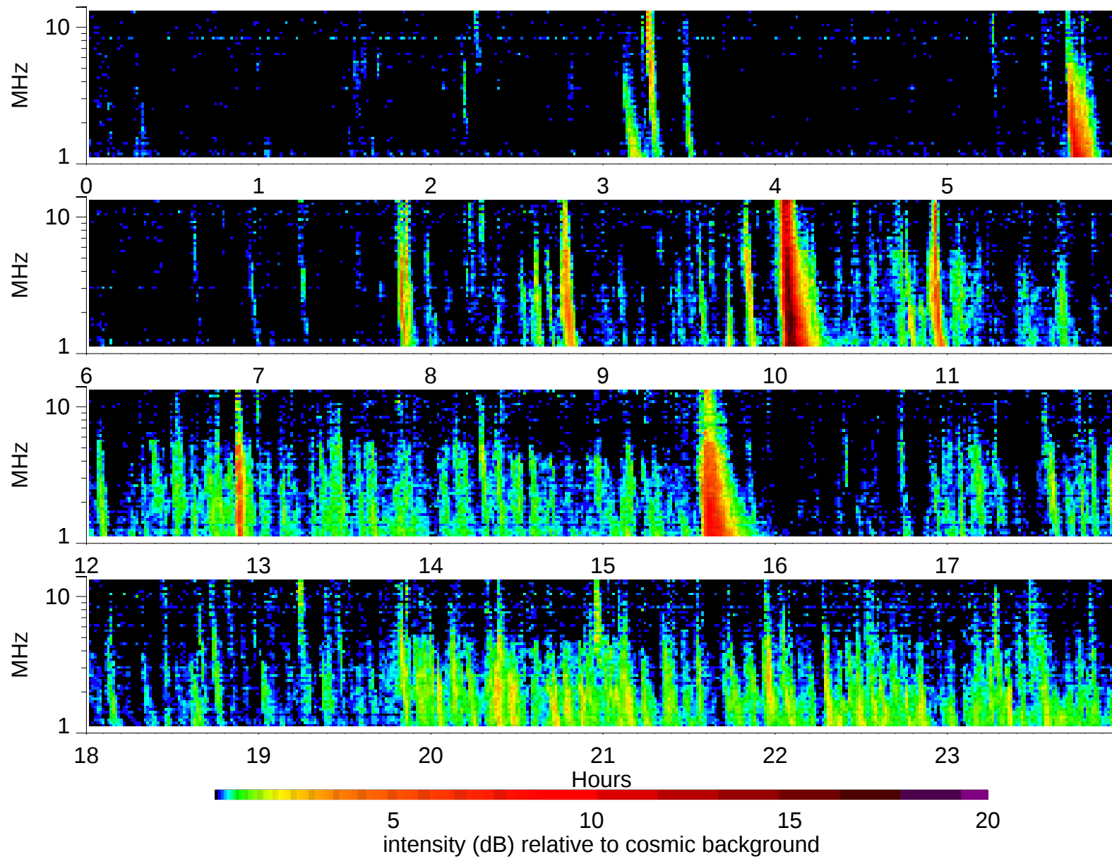
Wind Waves RAD2 receiver: 2003/3/10
