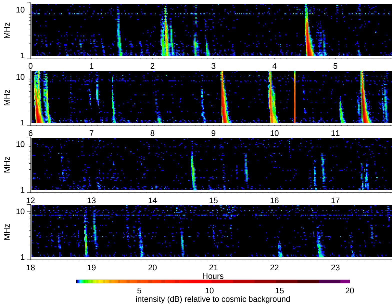
Wind Waves RAD2 receiver: 2003/3/8
