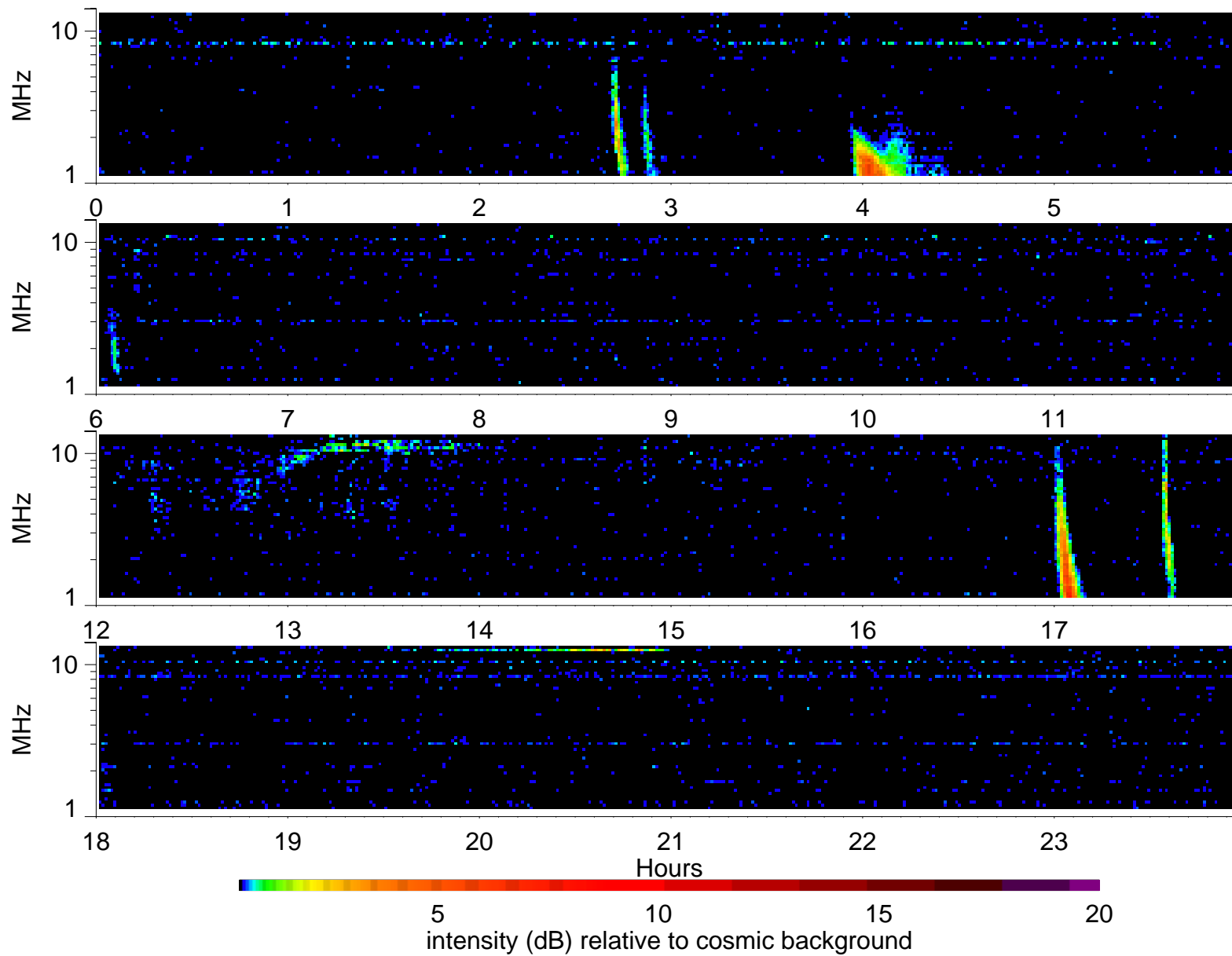
Wind Waves RAD2 receiver: 2003/3/4
