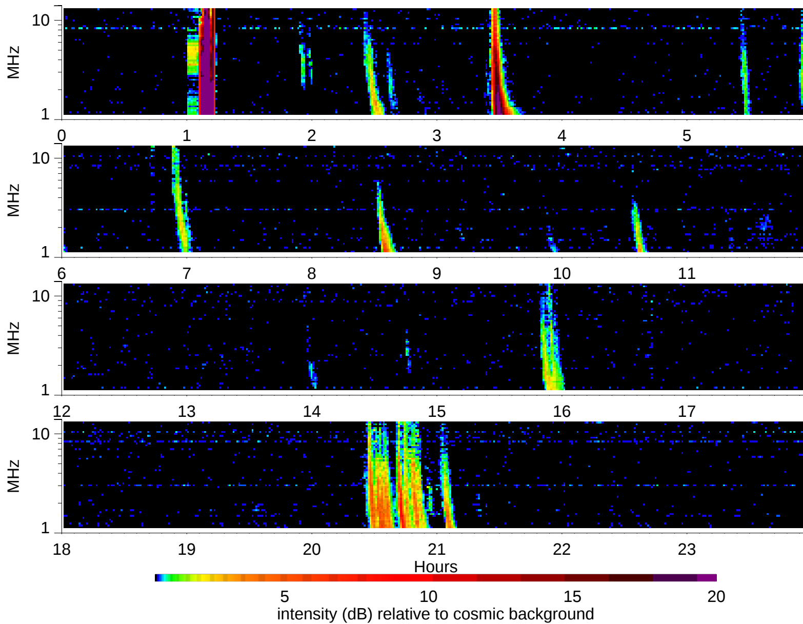
Wind Waves RAD2 receiver: 2003/3/3
