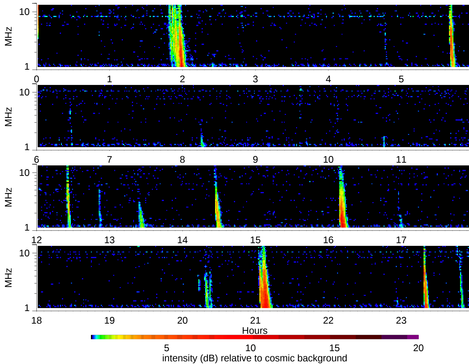
Wind Waves RAD2 receiver: 2003/2/12
