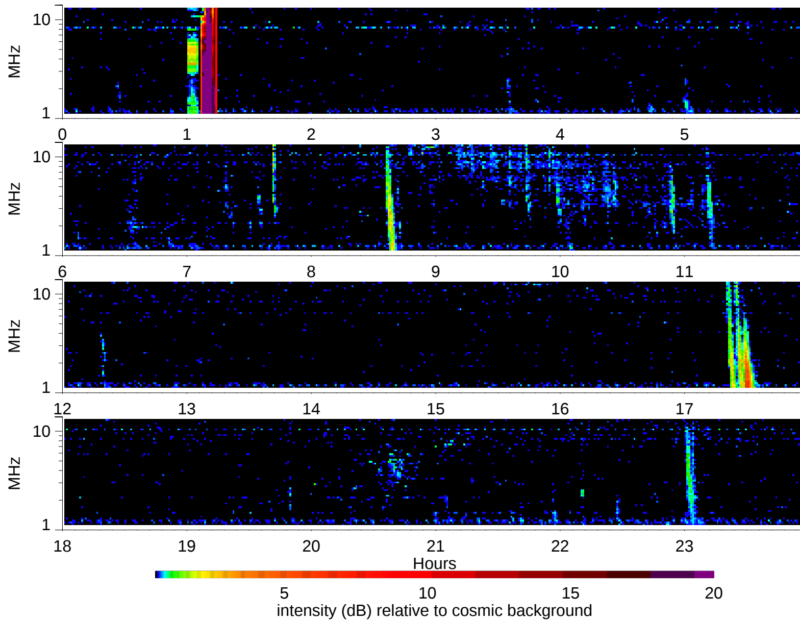
Wind Waves RAD2 receiver: 2003/2/11
