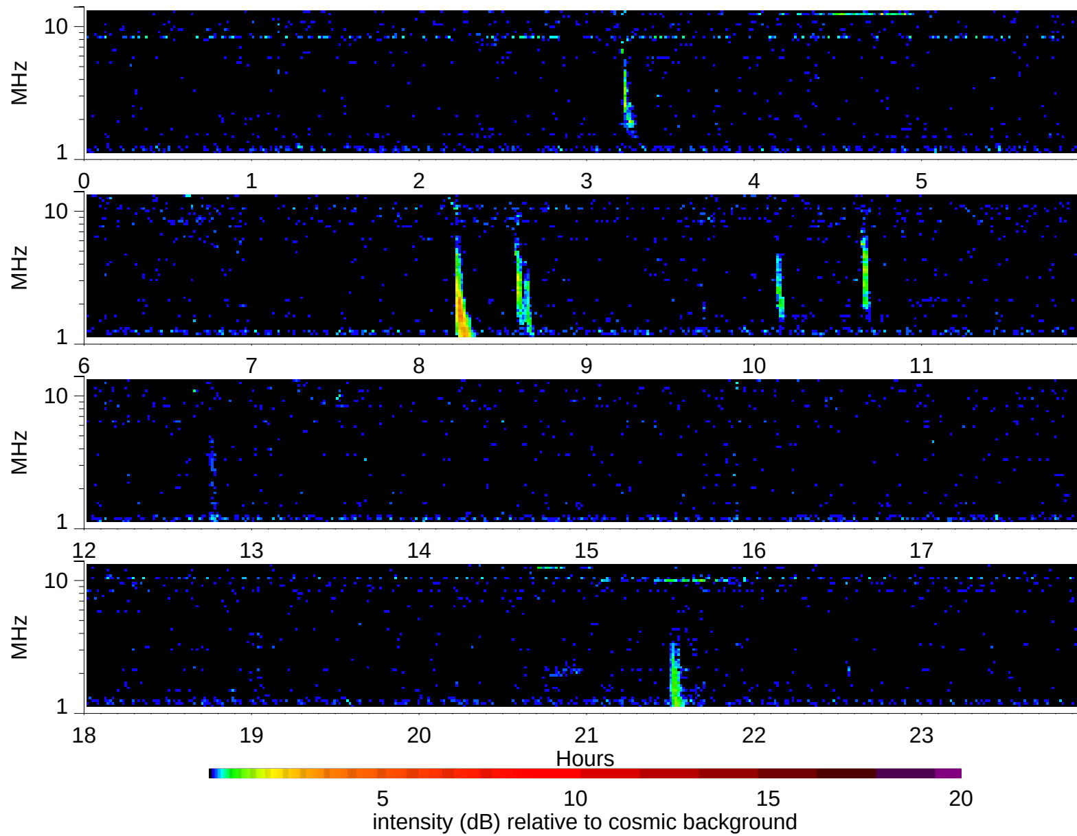
Wind Waves RAD2 receiver: 2003/2/10
