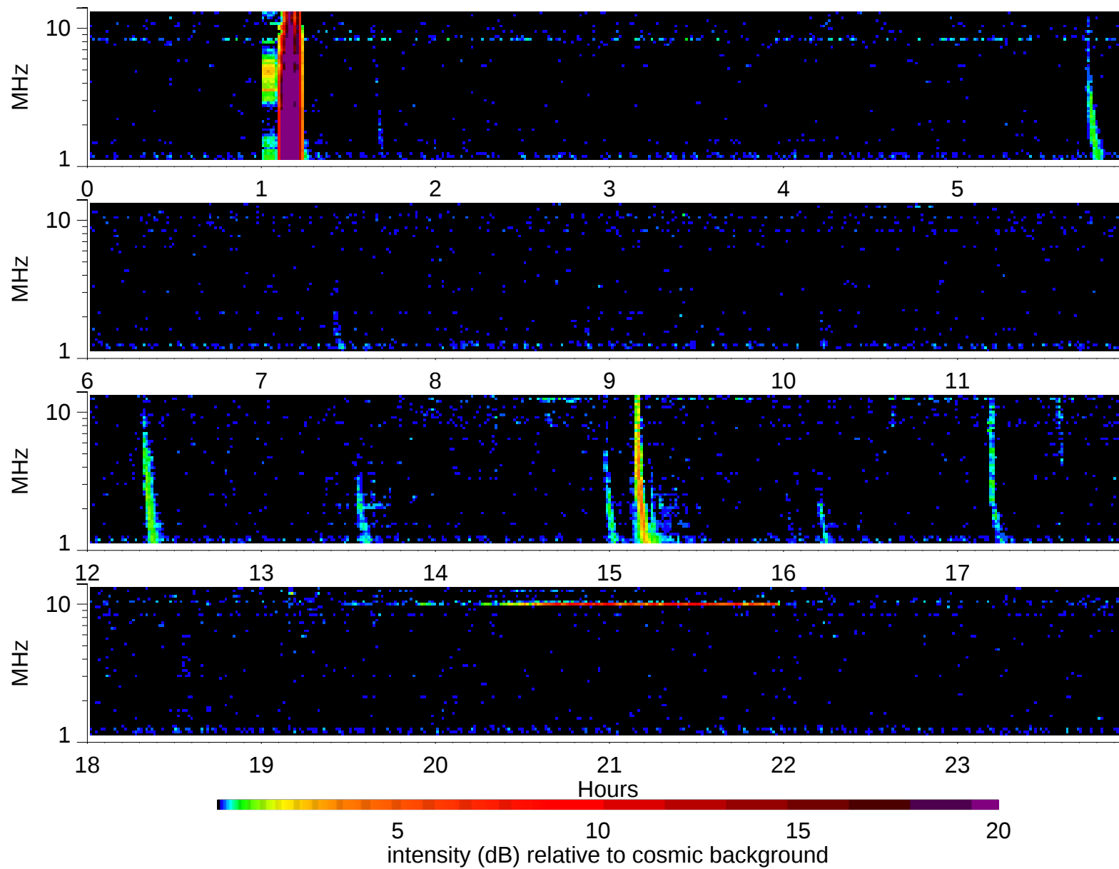
Wind Waves RAD2 receiver: 2003/2/7
