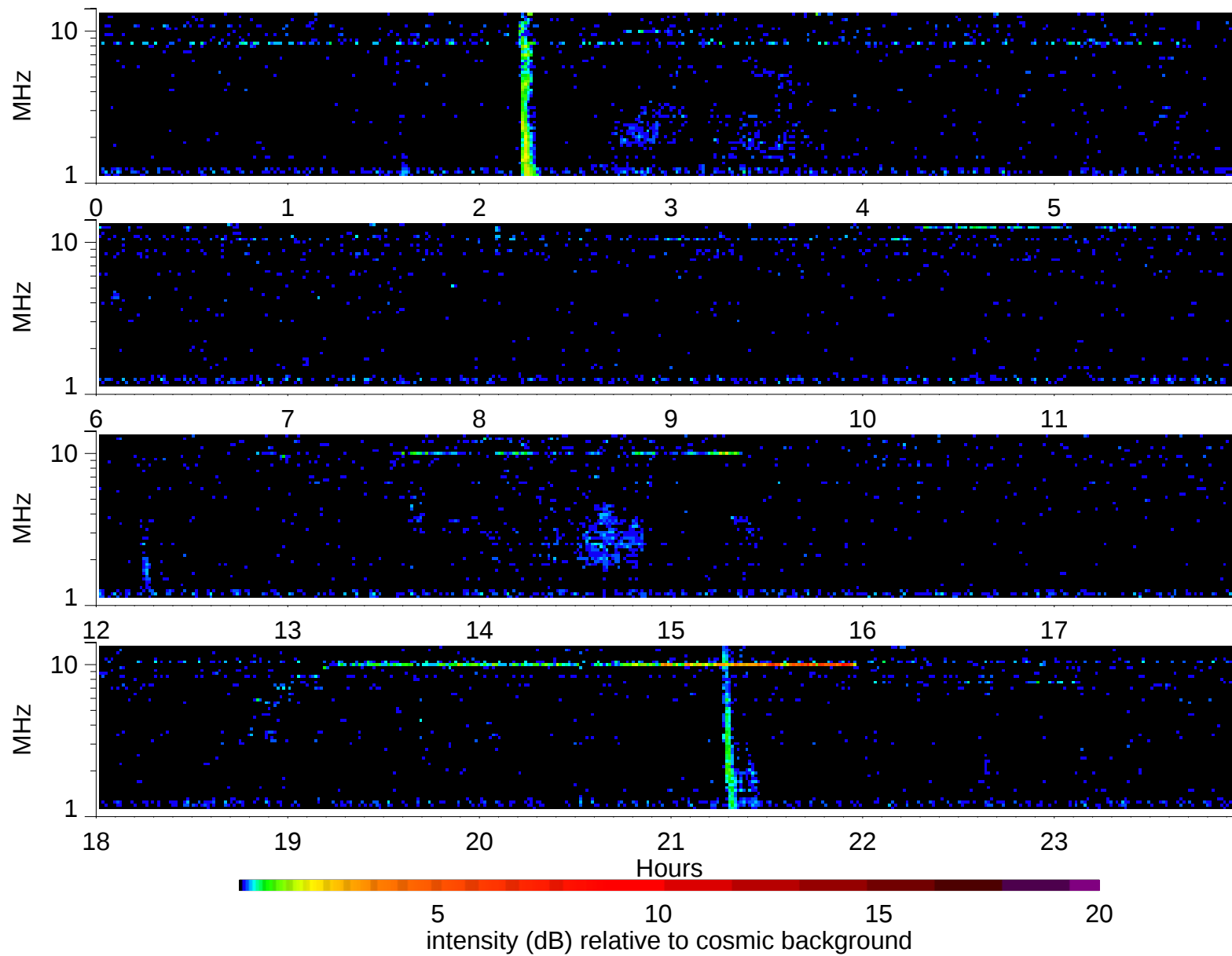
Wind Waves RAD2 receiver: 2003/2/4
