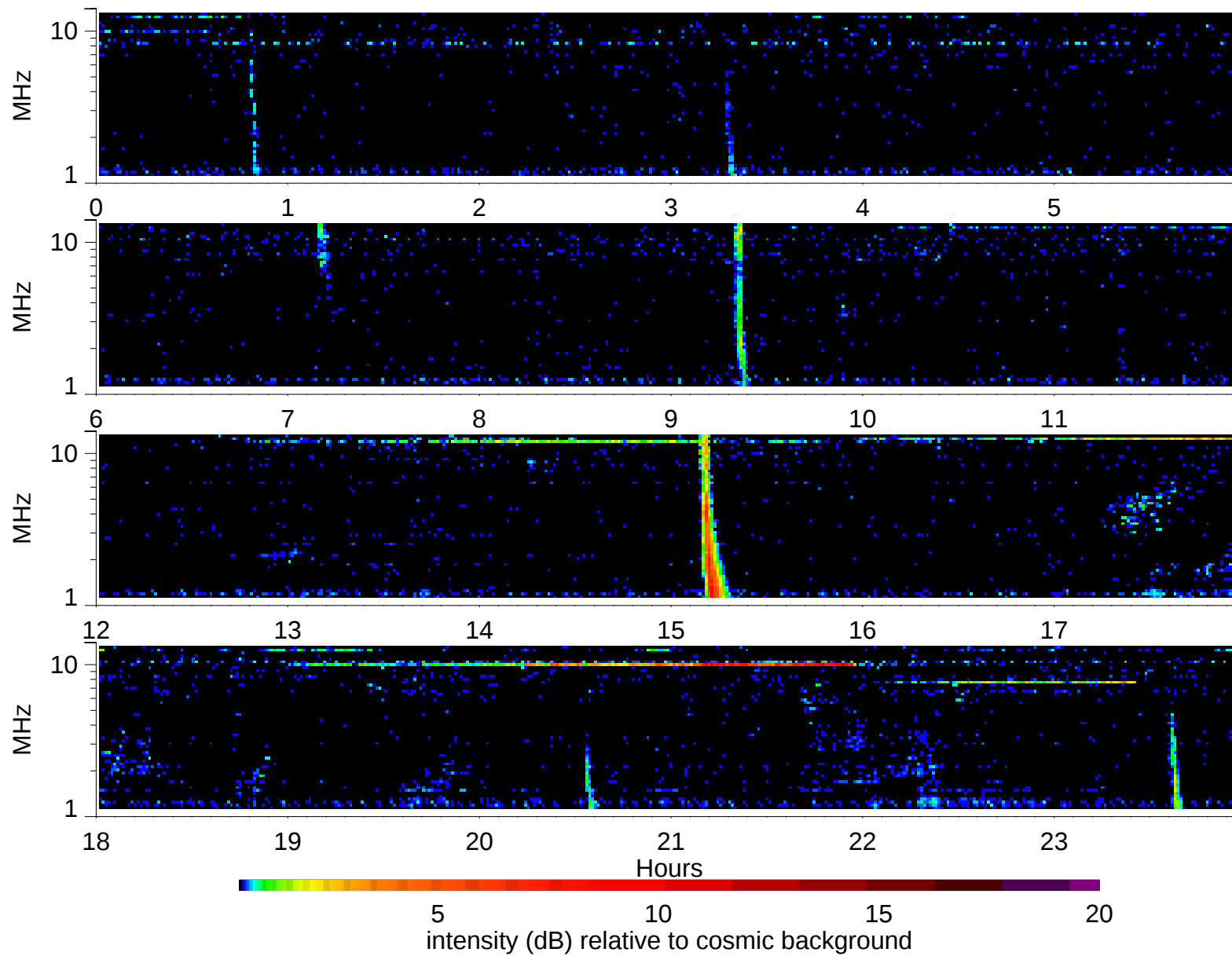
Wind Waves RAD2 receiver: 2003/1/31
