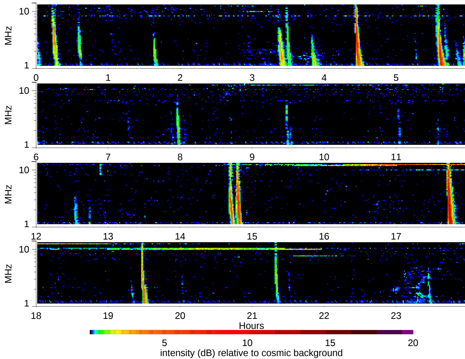
Wind Waves RAD2 receiver: 2003/1/19
