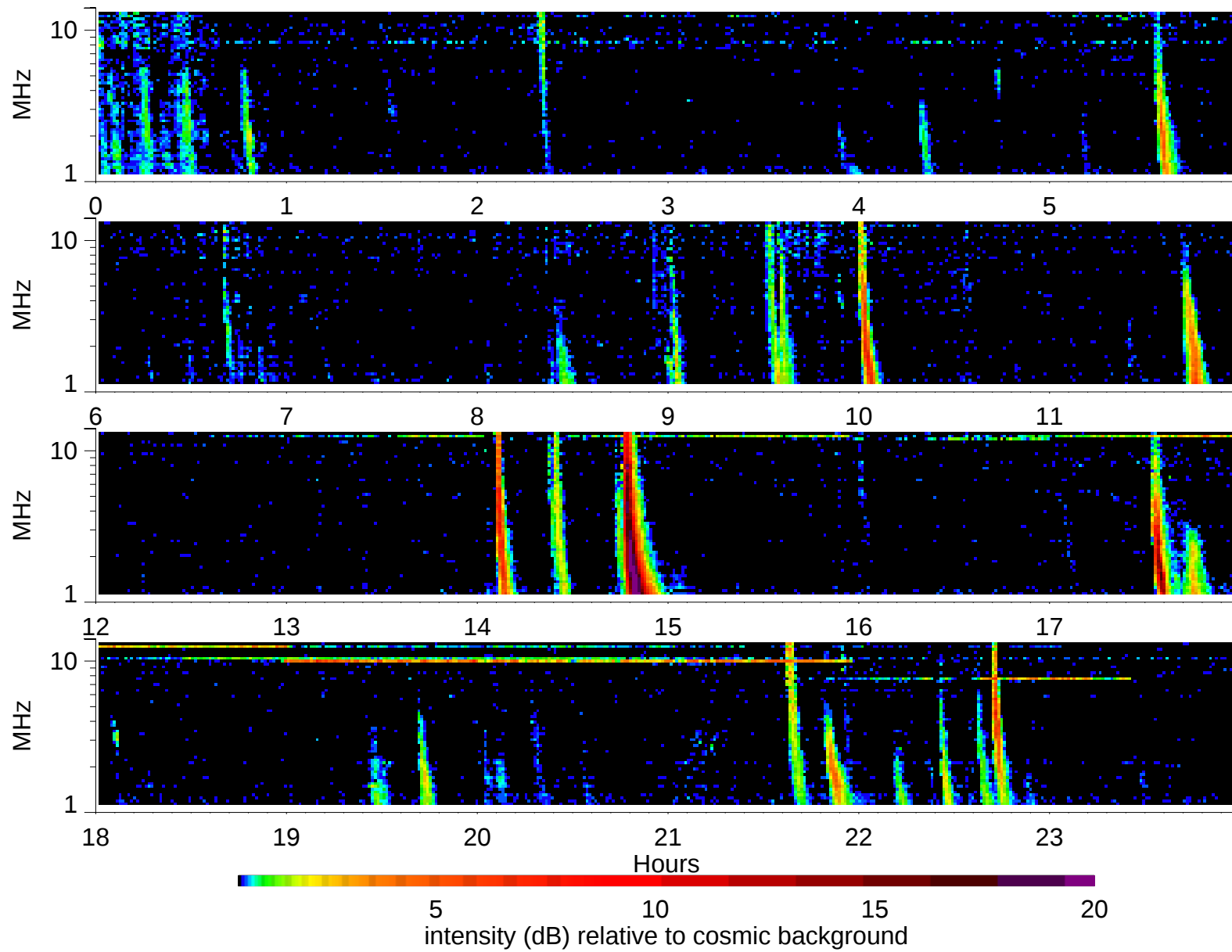
Wind Waves RAD2 receiver: 2003/1/11
