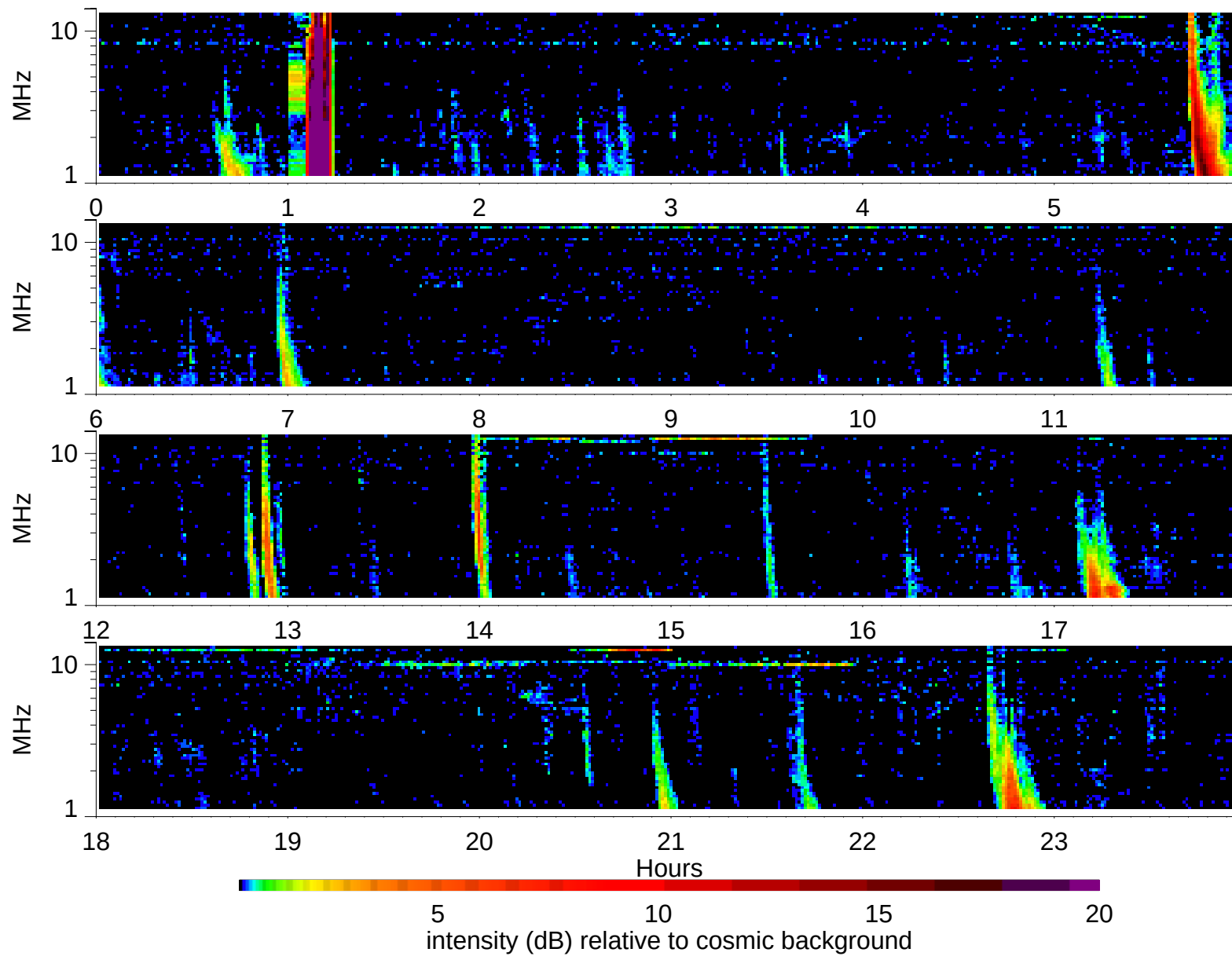
Wind Waves RAD2 receiver: 2003/1/8
