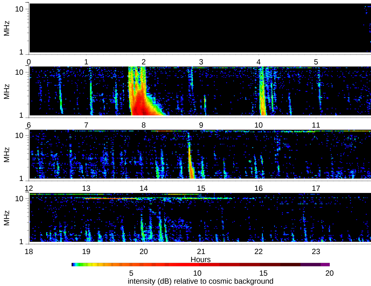
Wind Waves RAD2 receiver: 2003/1/7
