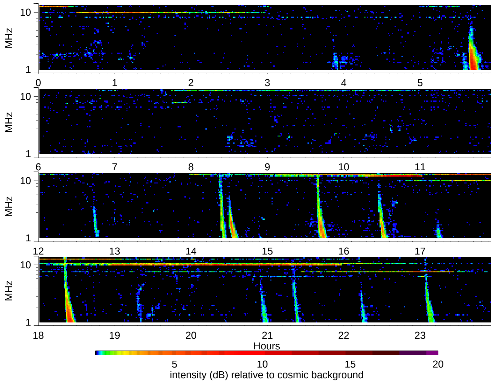
Wind Waves RAD2 receiver: 2003/1/3
