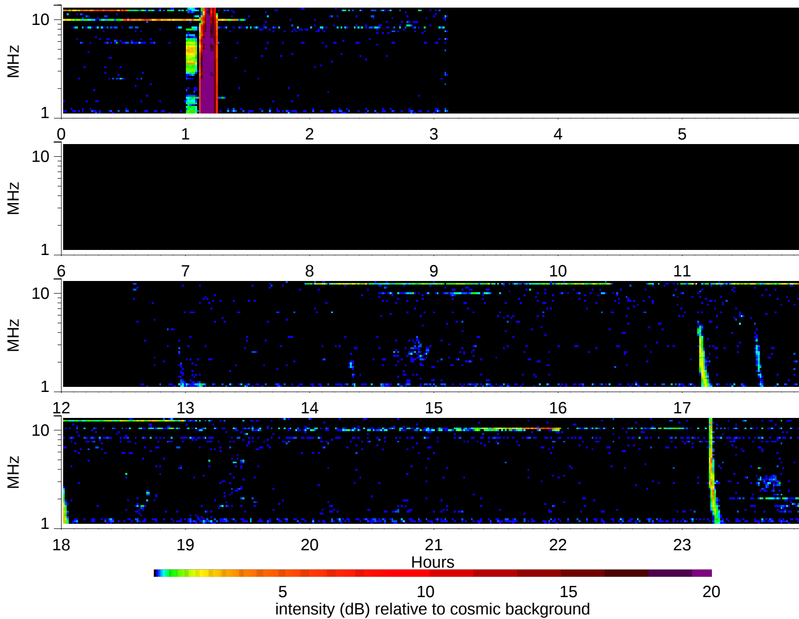
Wind Waves RAD2 receiver: 2003/1/2
