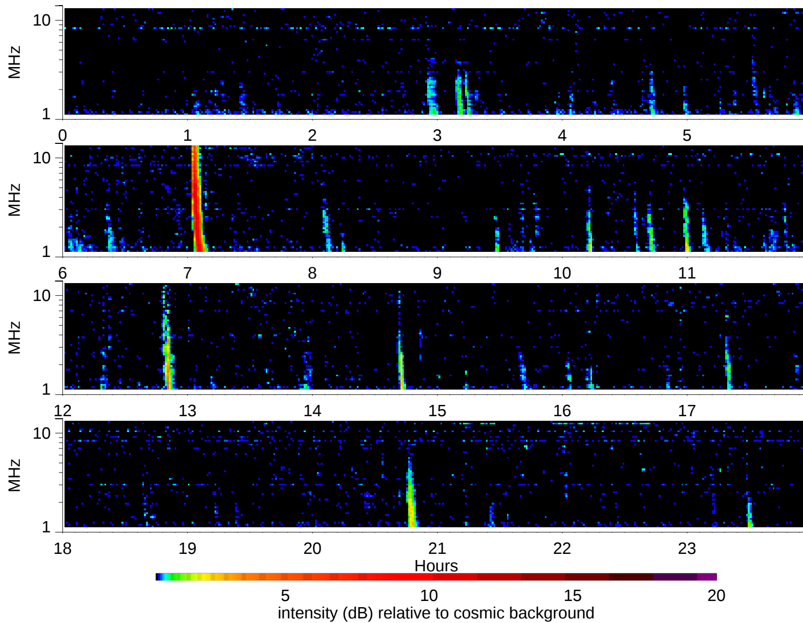
Wind Waves RAD2 receiver: 2002/10/16
