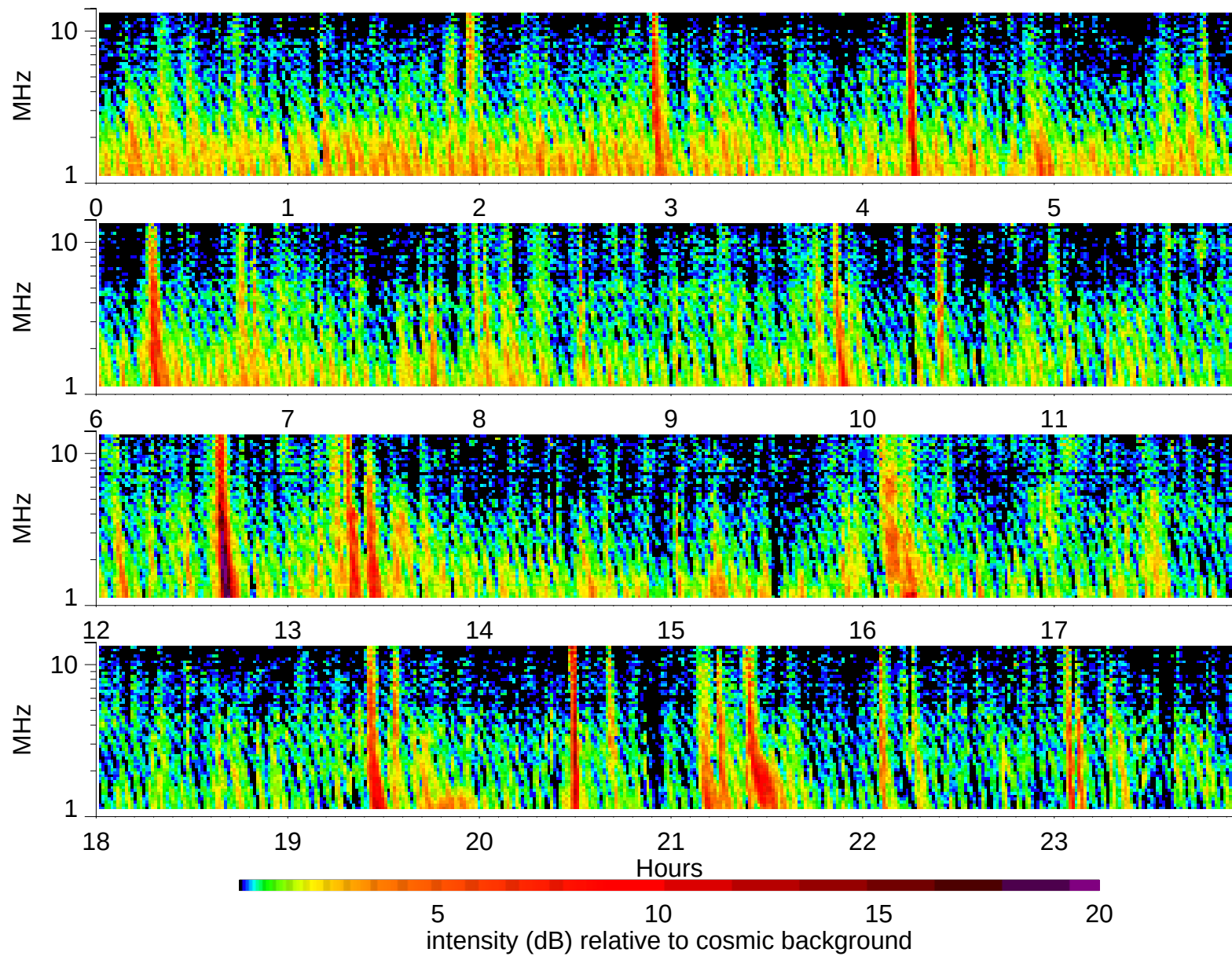
Wind Waves RAD2 receiver: 2002/9/20
