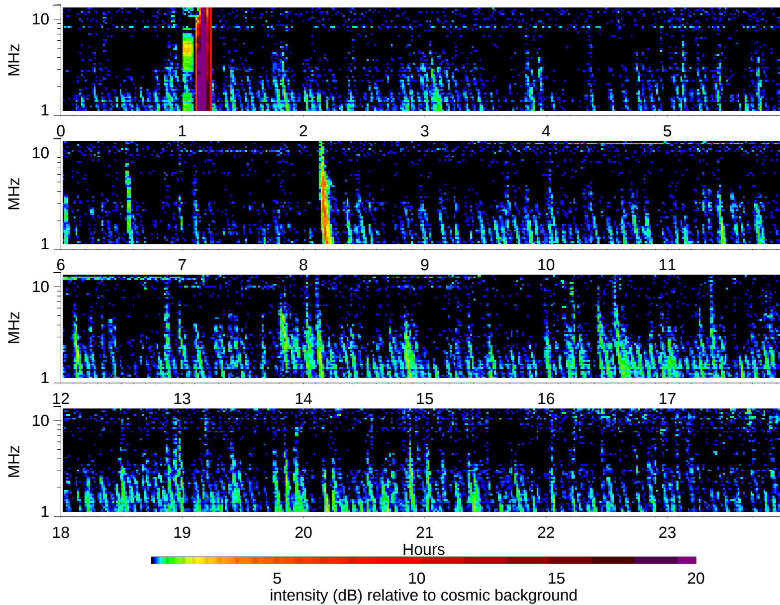
Wind Waves RAD2 receiver: 2002/9/11
