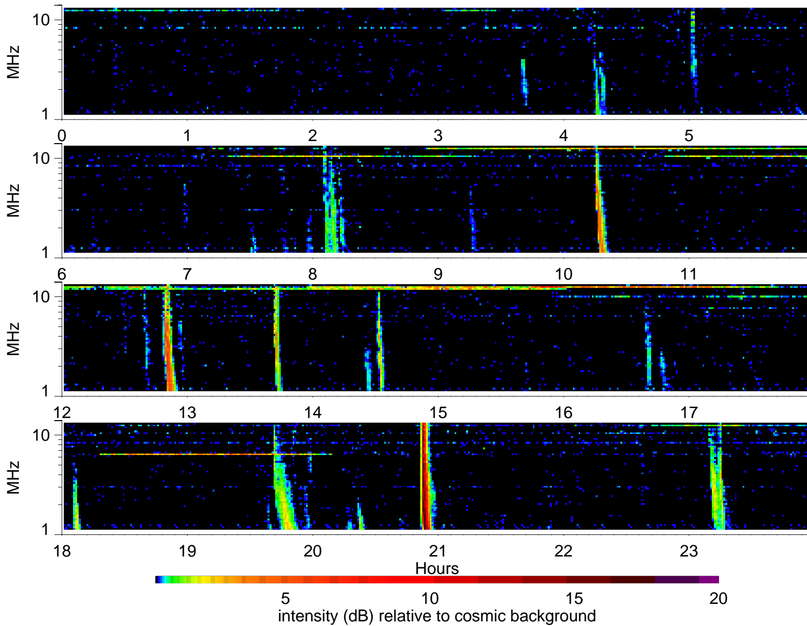
Wind Waves RAD2 receiver: 2002/6/18
