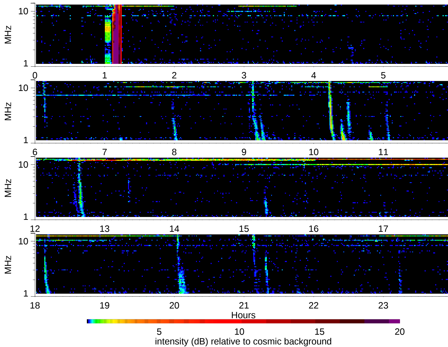
Wind Waves RAD2 receiver: 2002/6/11
