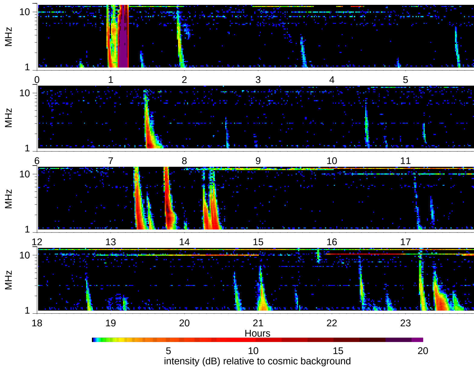
Wind Waves RAD2 receiver: 2002/5/14
