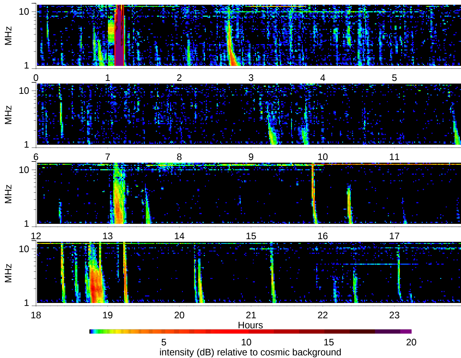
Wind Waves RAD2 receiver: 2002/5/8
