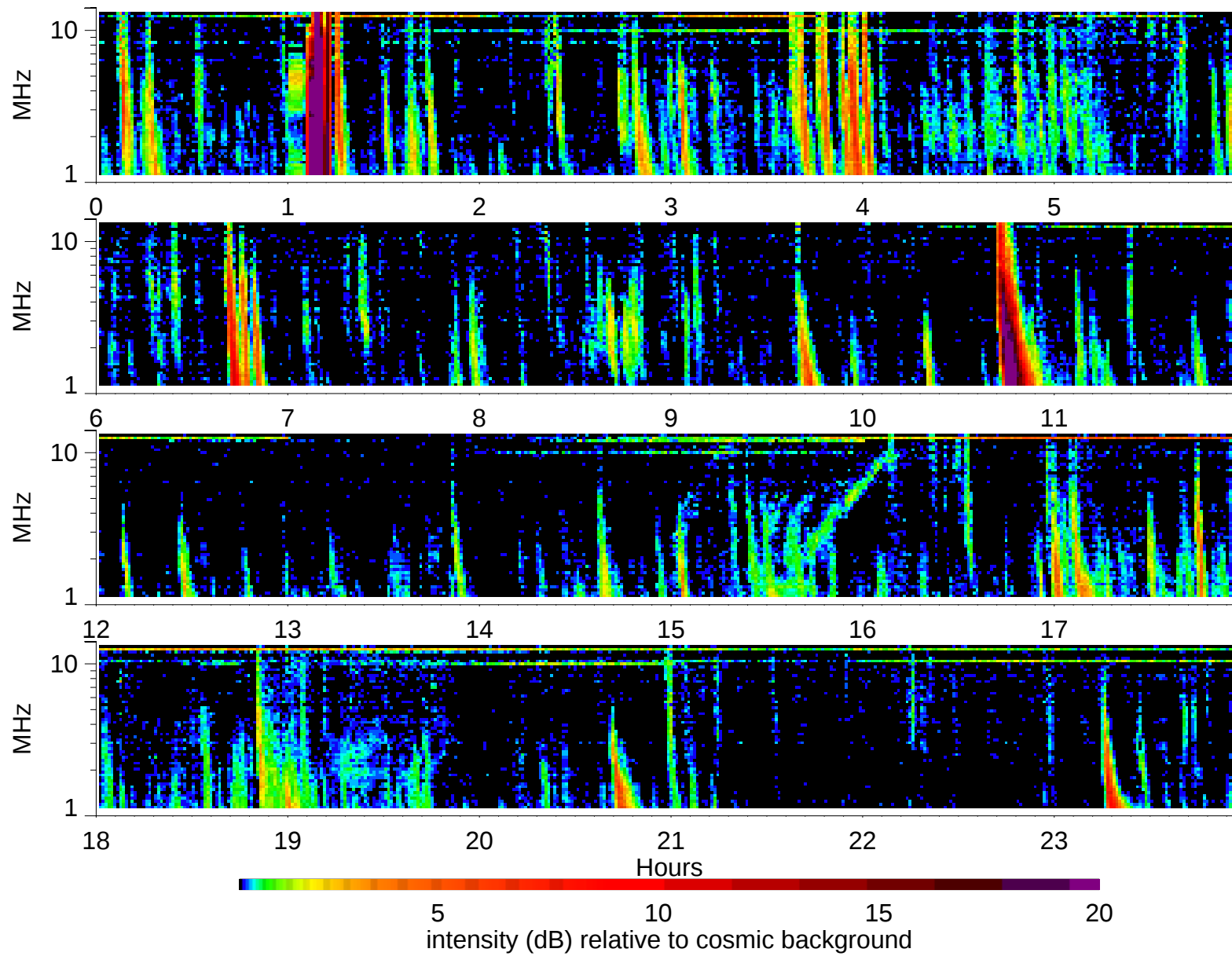
Wind Waves RAD2 receiver: 2002/4/16
