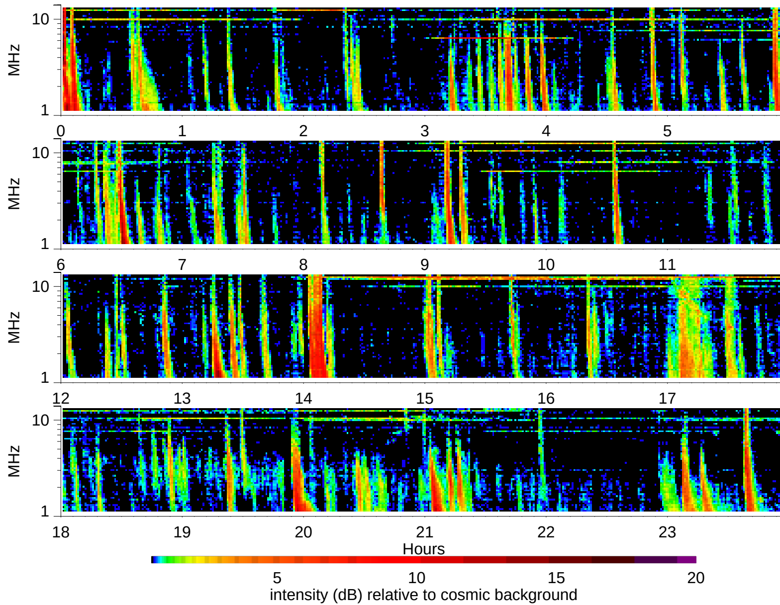
Wind Waves RAD2 receiver: 2002/3/20
