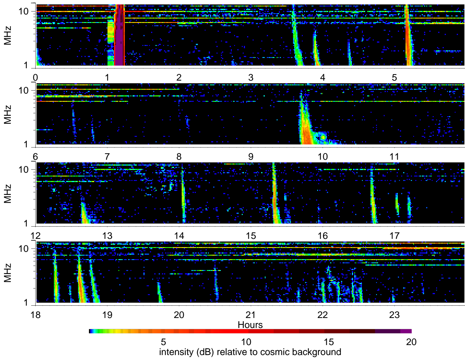
Wind Waves RAD2 receiver: 2002/1/4
