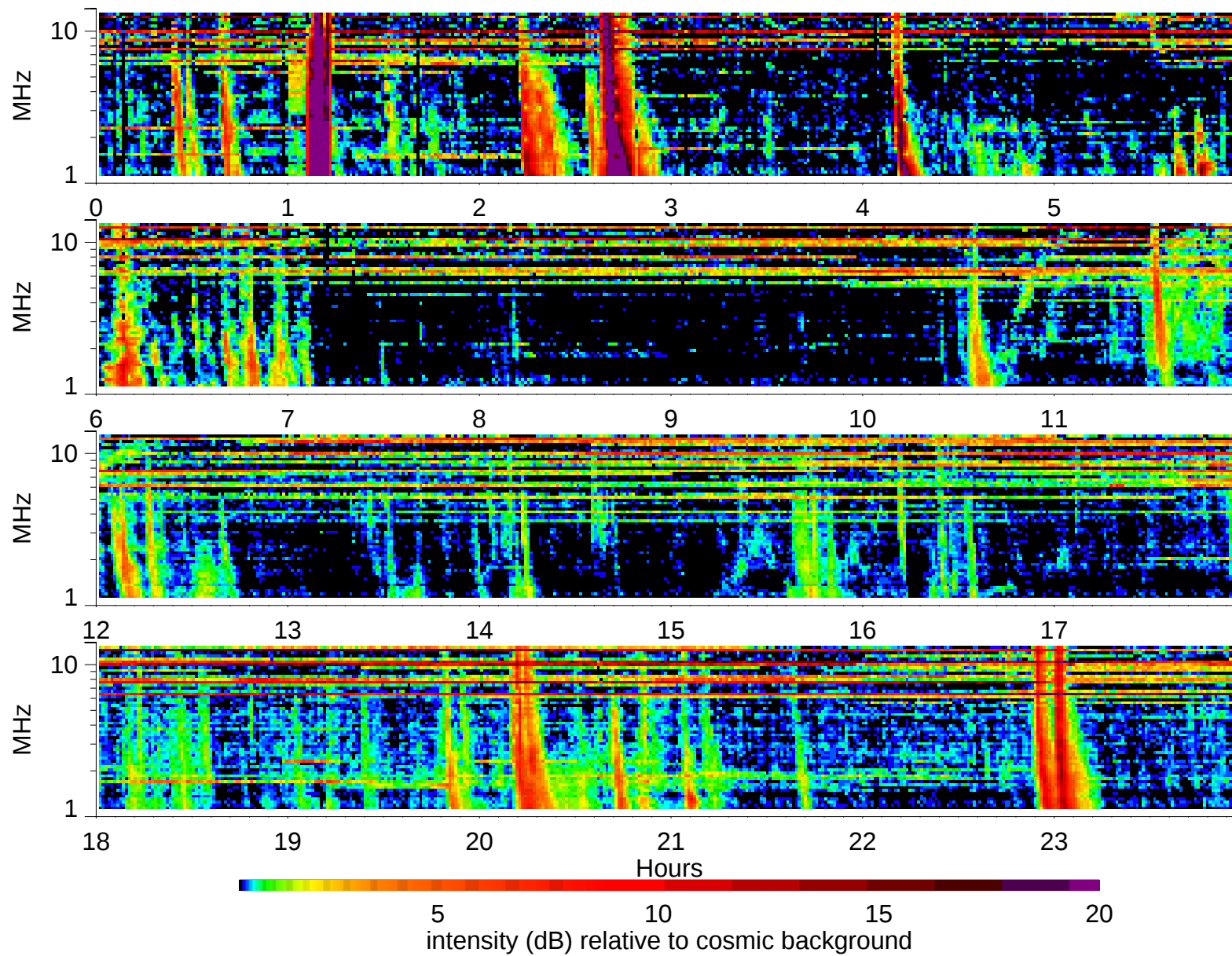
Wind Waves RAD2 receiver: 1999/11/16
