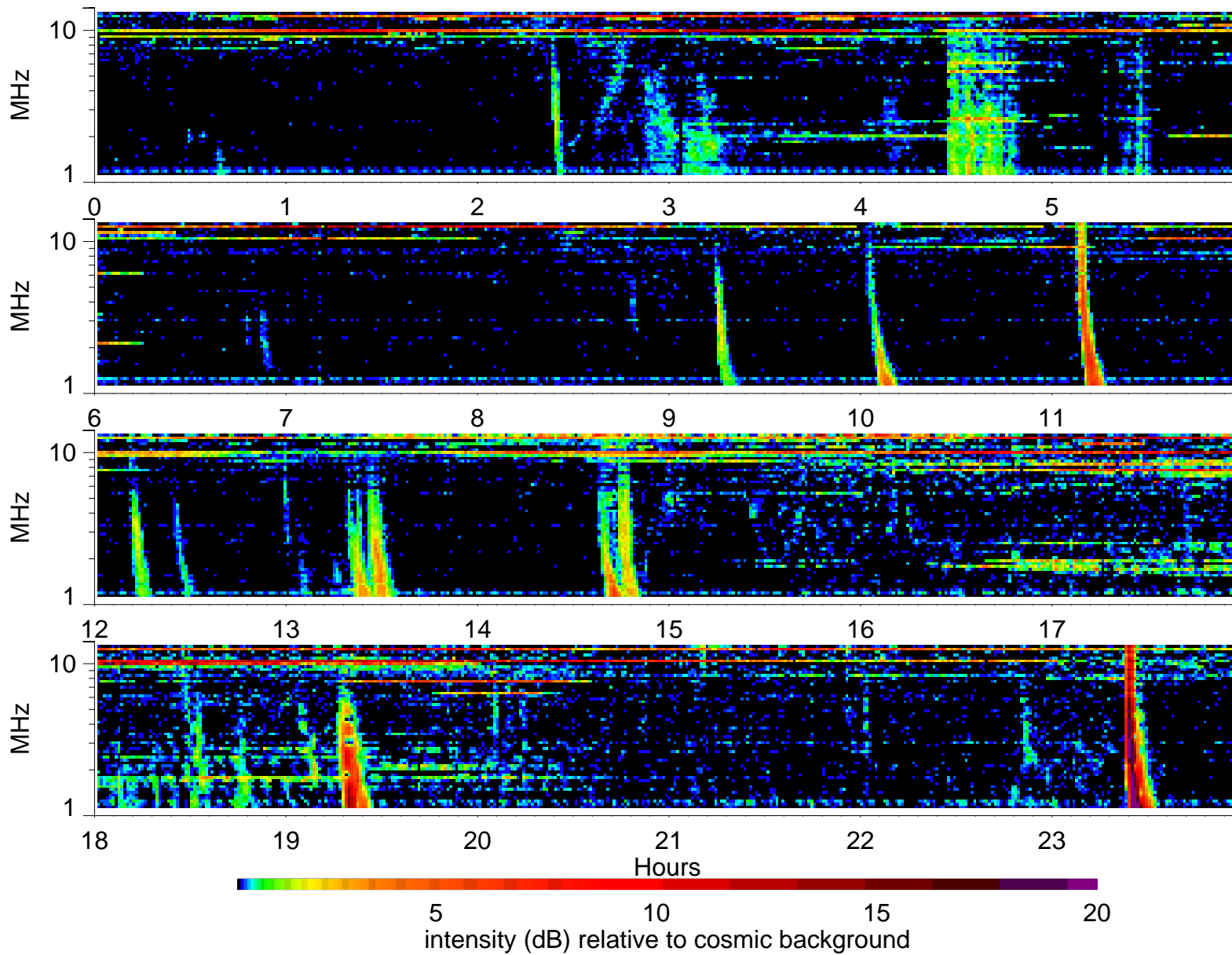
Wind Waves RAD2 receiver: 1999/10/12
