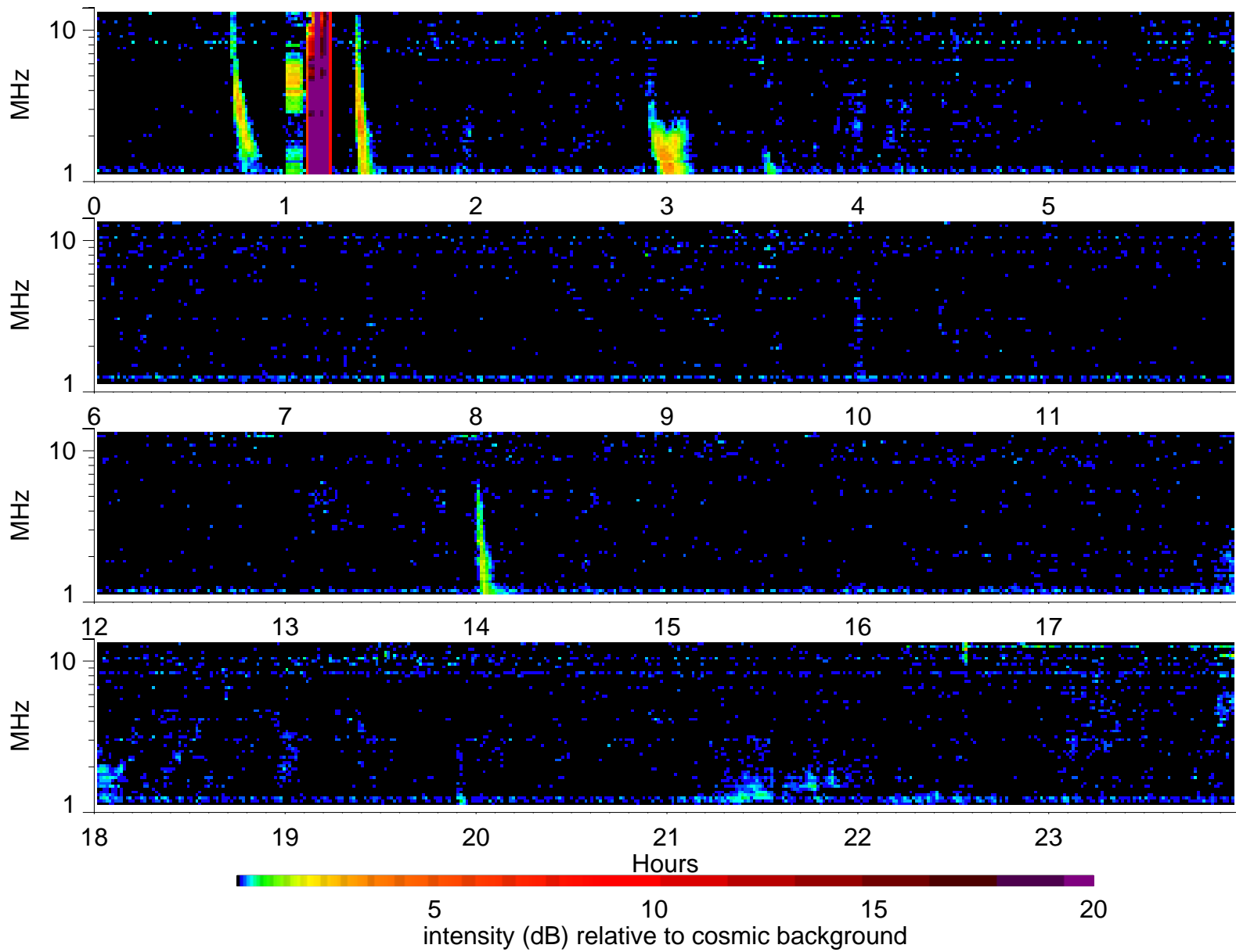
Wind Waves RAD2 receiver: 1999/9/5
