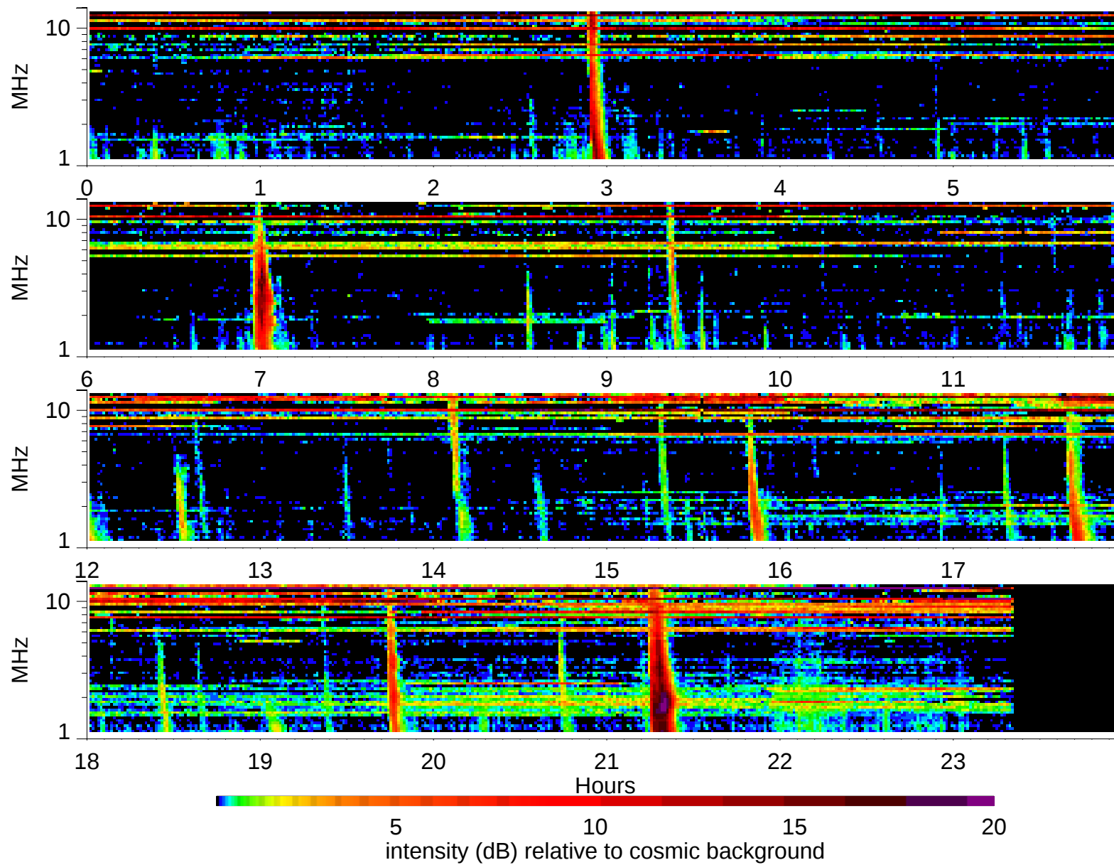
Wind Waves RAD2 receiver: 1999/5/7
