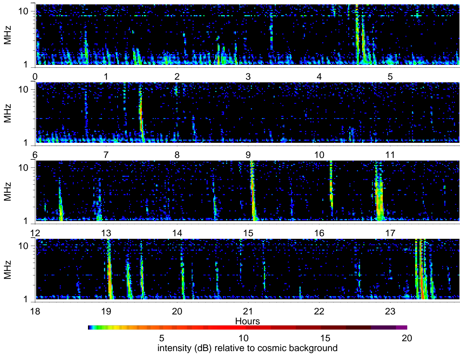
Wind Waves RAD2 receiver: 1998/11/11
