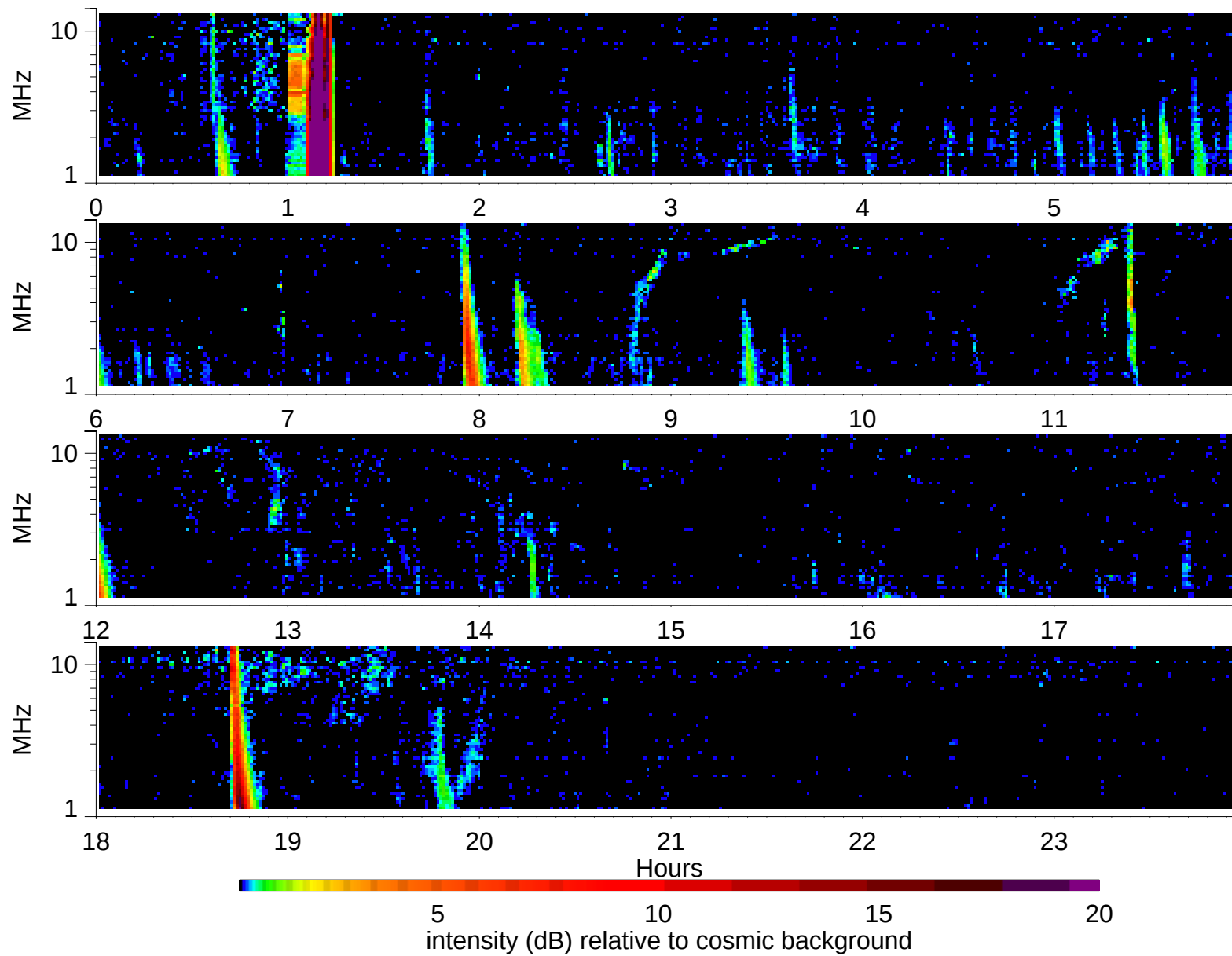
Wind Waves RAD2 receiver: 1998/10/13
