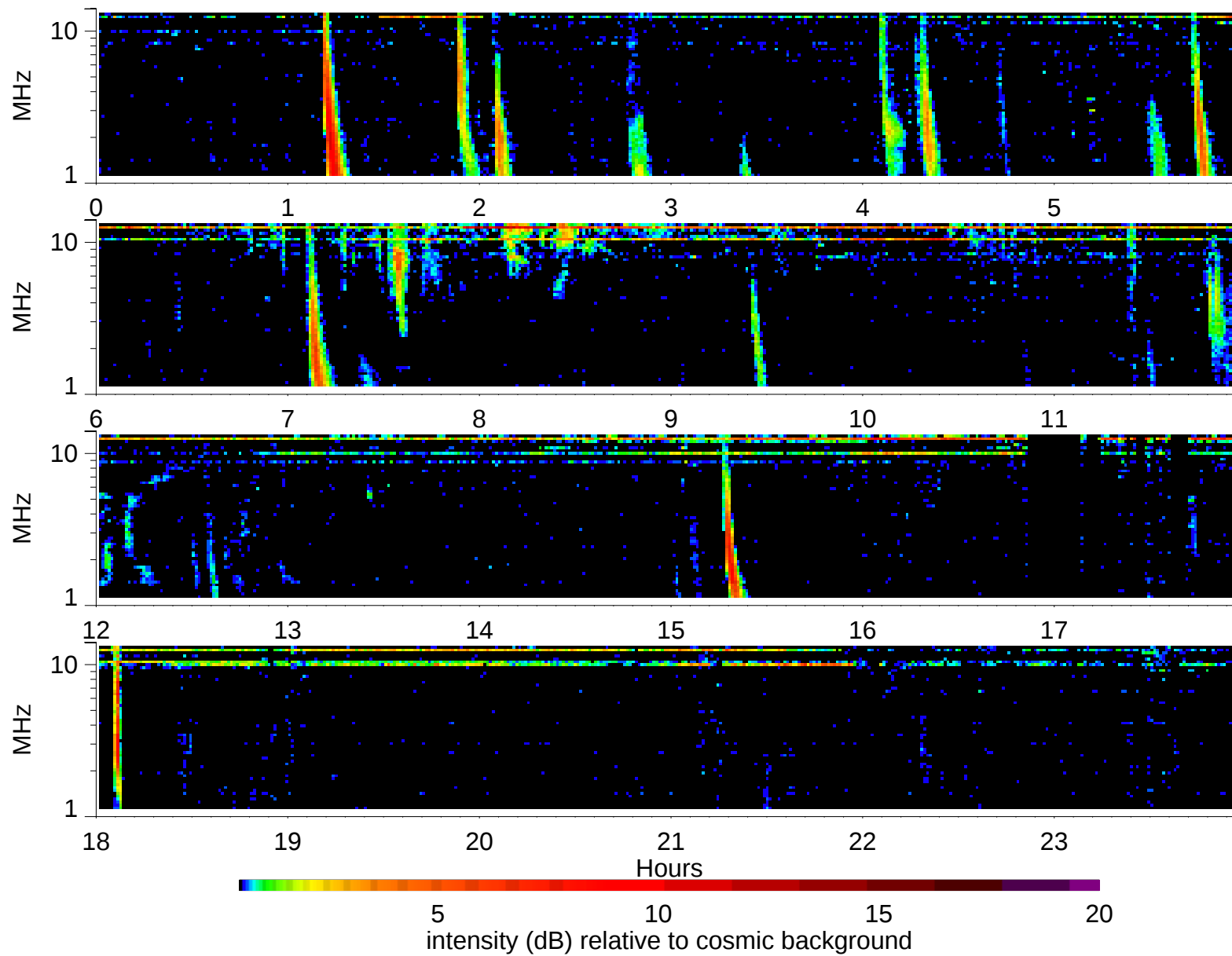
Wind Waves RAD2 receiver: 1998/6/10
