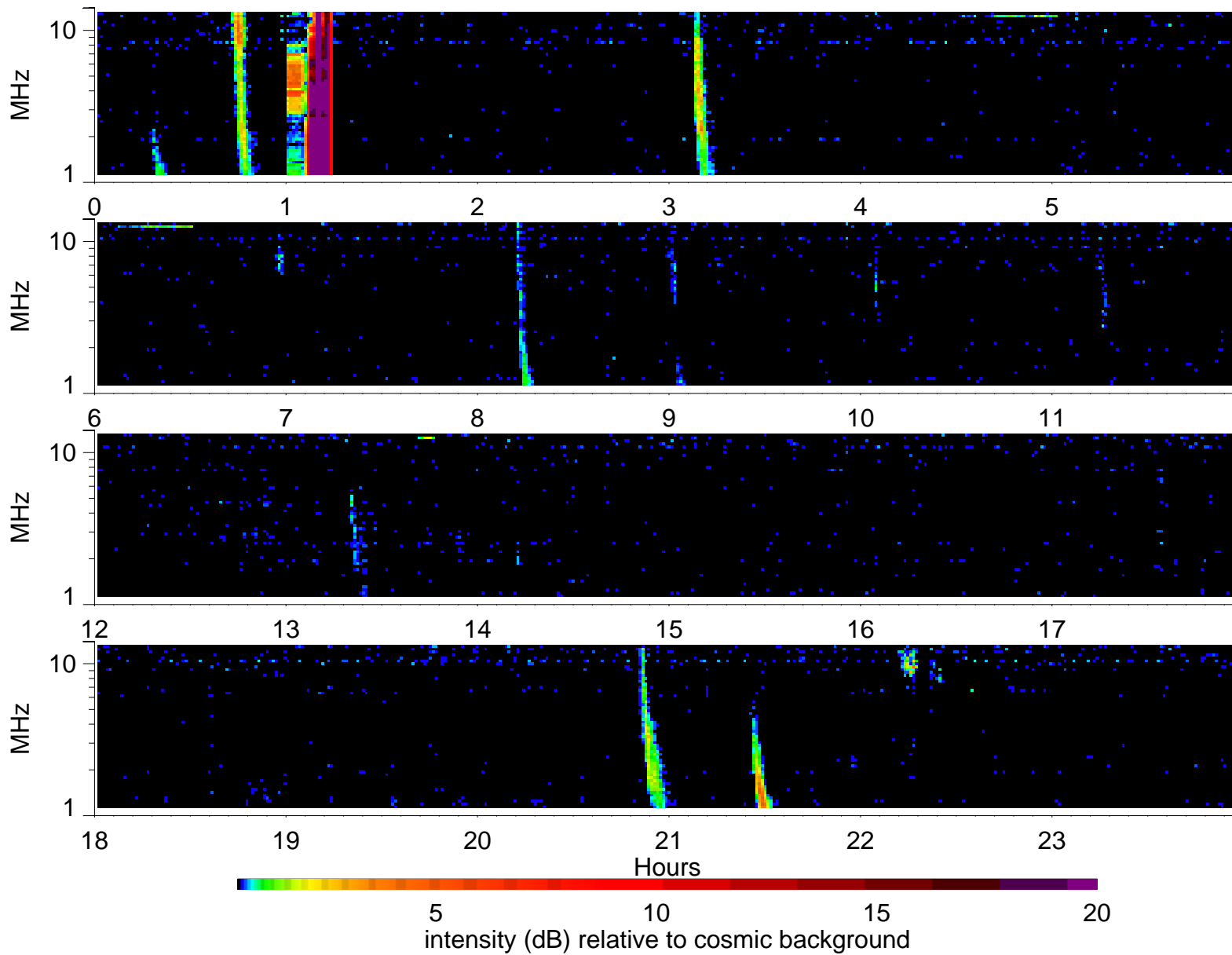
Wind Waves RAD2 receiver: 1998/2/23
