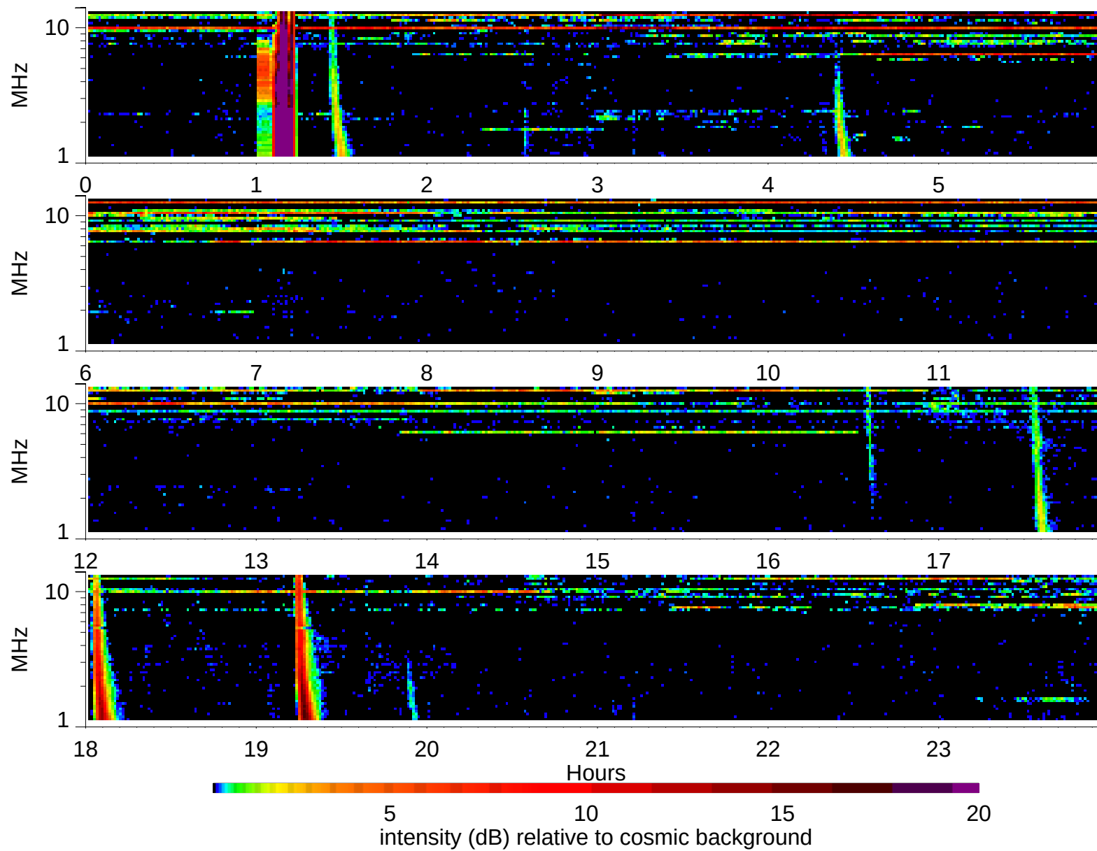
Wind Waves RAD2 receiver: 1997/8/10
