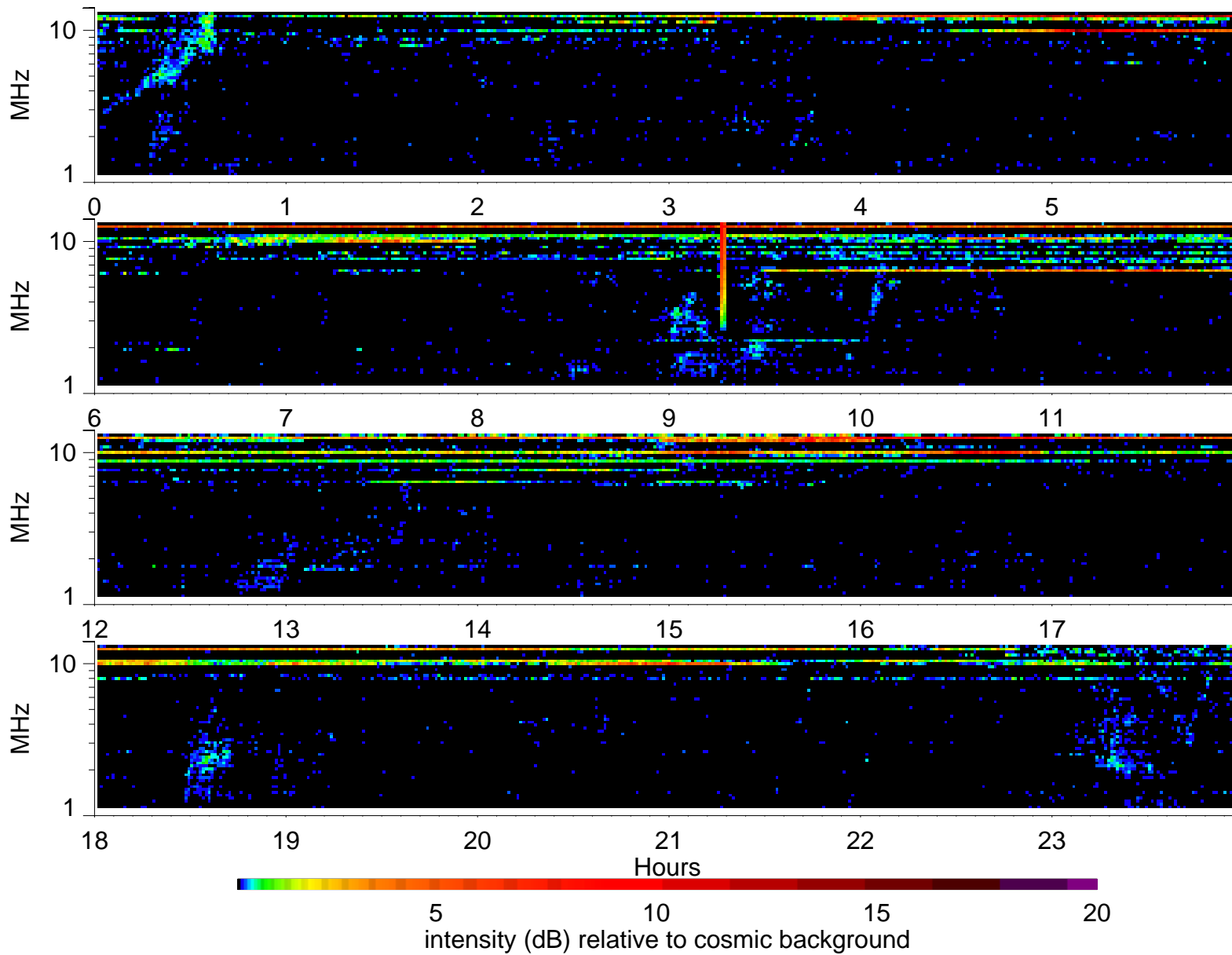
Wind Waves RAD2 receiver: 1997/5/31
