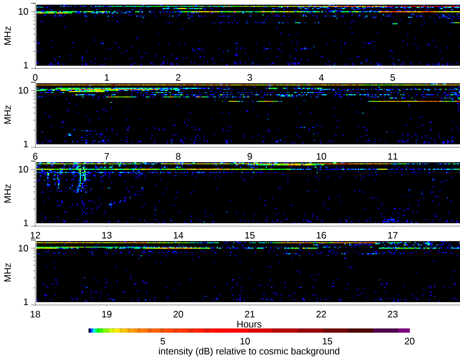
Wind Waves RAD2 receiver: 1997/5/11
