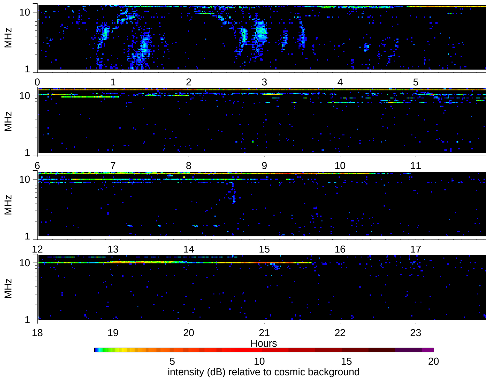
Wind Waves RAD2 receiver: 1997/3/20
