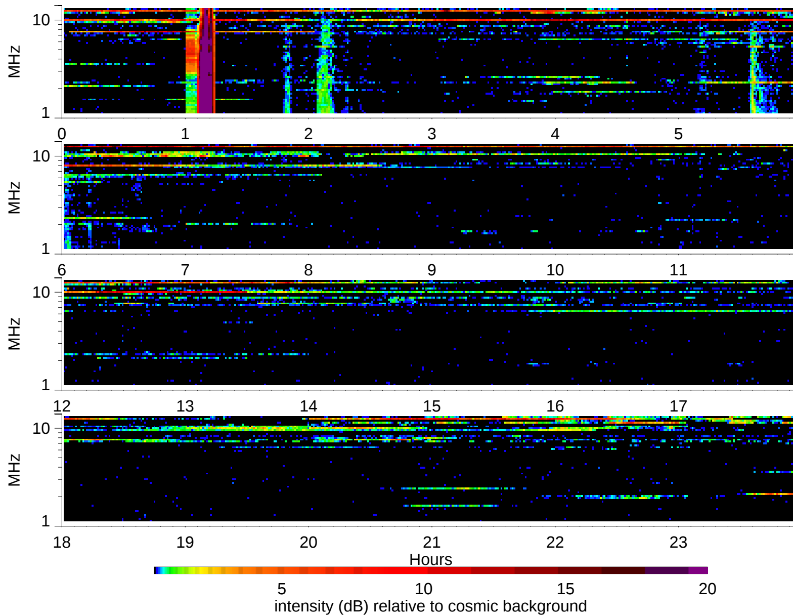
Wind Waves RAD2 receiver: 1995/12/28
