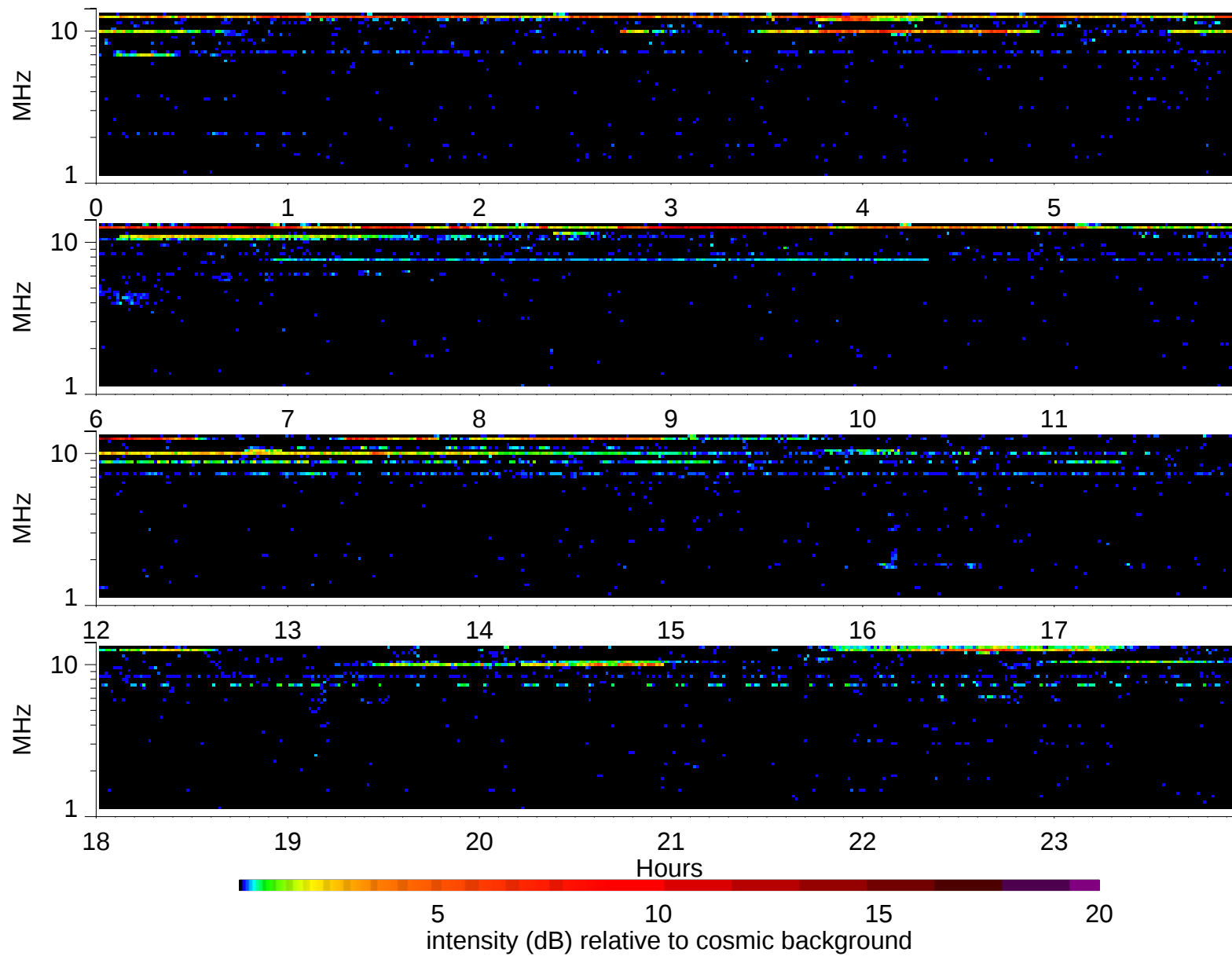
Wind Waves RAD2 receiver: 1995/12/3
