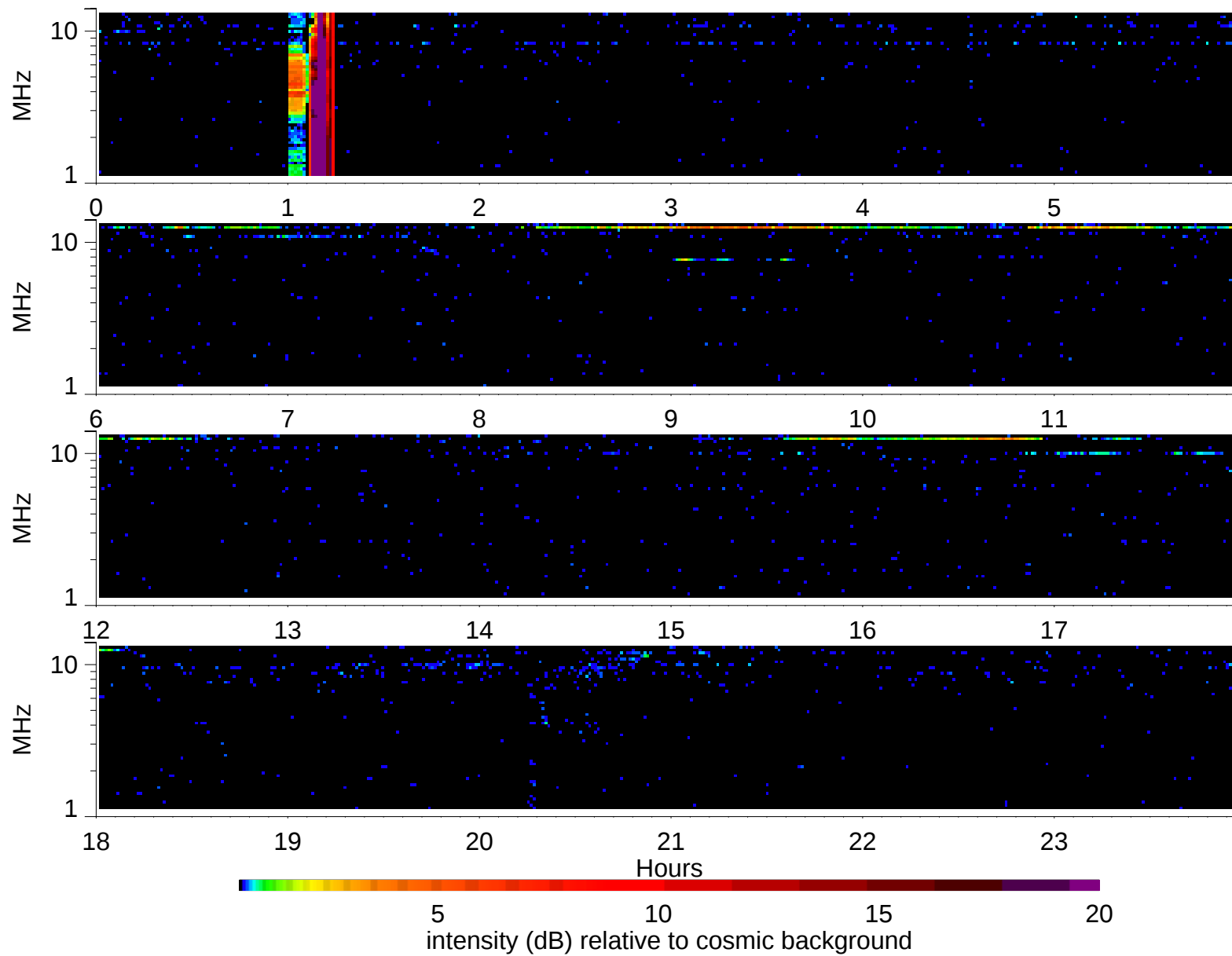
Wind Waves RAD2 receiver: 1995/10/25
